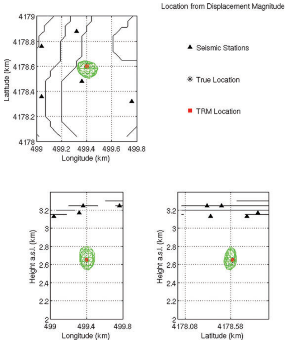
Figure 5. Time reverse source location and true location for the second synthetic data set (vertical force source). The hashed volume is the 95 per cent of the maximum displacement contour. In this test the source is non-isotropic giving rise to the oblong source region. The black lines are elevation contours.
