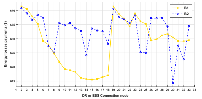
Fig. 6. The energy losses payments in loss minimization strategy vs the ESS node (case B_1 ) and DR node (case B_2 ).
