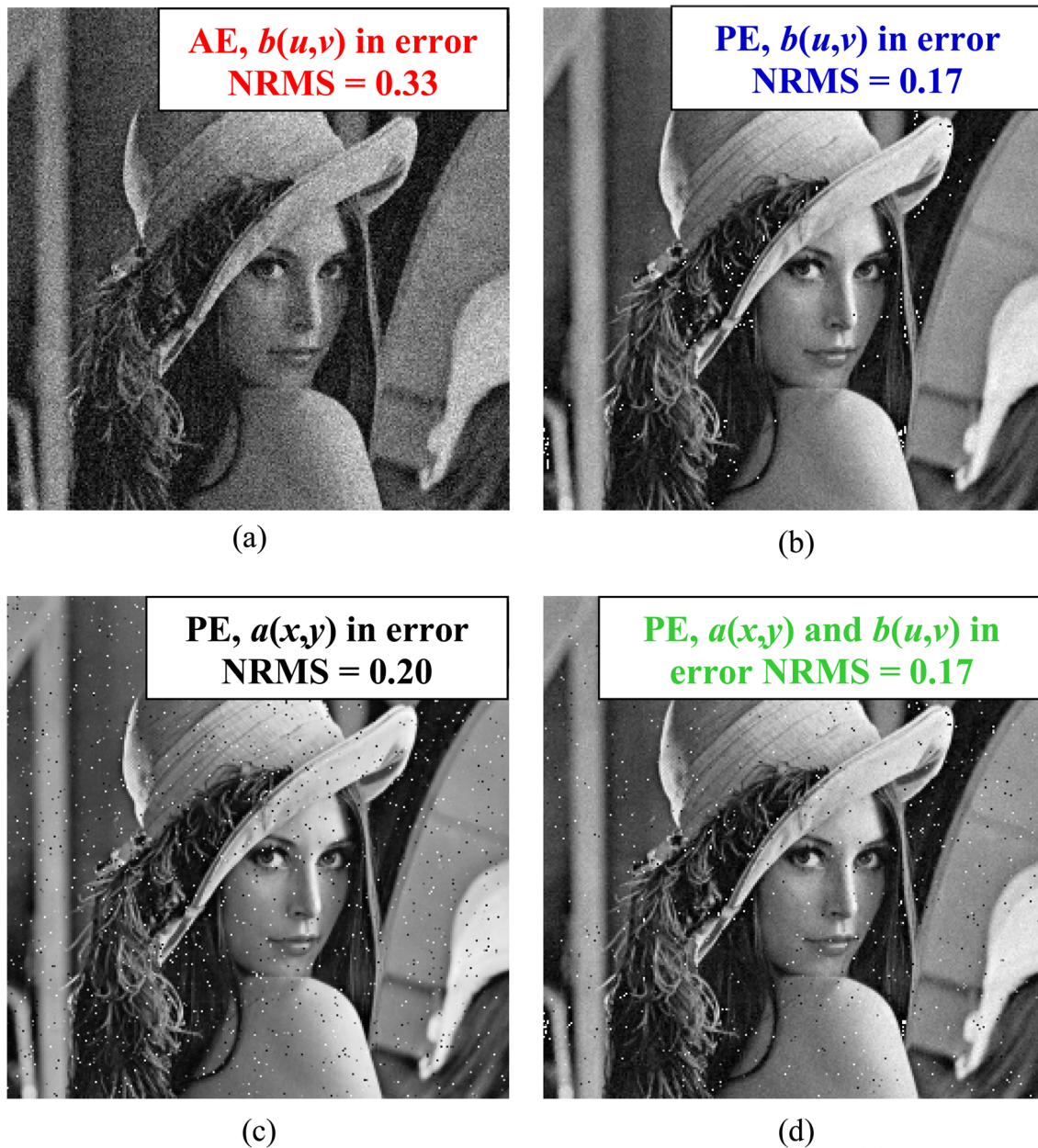
Fig. 6. (Color online) Results when 2.59% of phase key pixels are in error. (a) AE case with R2 in error and \text{NRMS} \sim 0.33 . (b)–(d) PE case with a \text{NRMS} of (b) 0.17, (c) 0.20, and (d) 0.17. In (b) R2 is in error. In (c) R1 is in error, and in (d) both R1 and R2 are in error.
