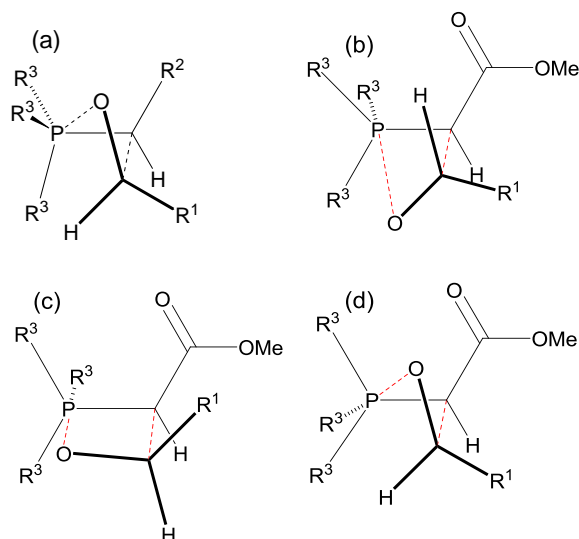
Figure 2. Proposed [2+2] cycloaddition transition states for various Wittig reactions.
