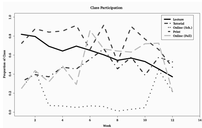
Figure 4: Proportion of students attending lectures, tutorials, or engaging with online materials, by week.
