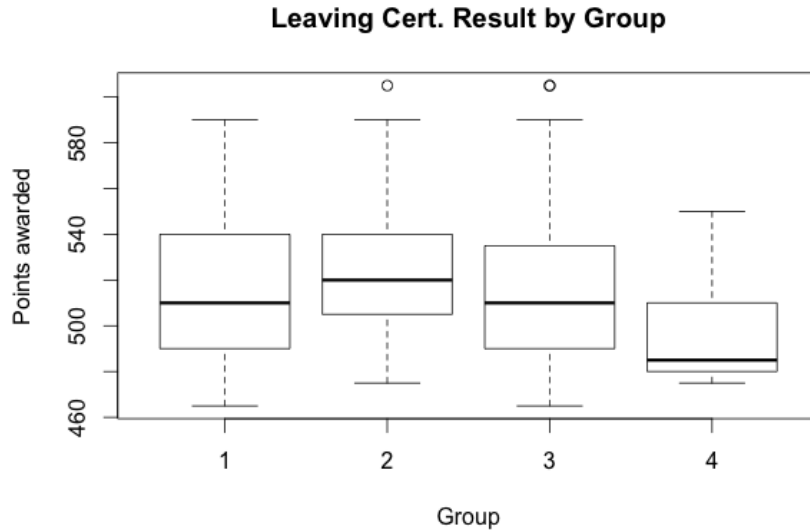
Figure 9: Boxplot of Leaving Cert. results by cluster. Note that the majority (approx. 75%) of students in Group 4 performed worse than the median scores achieved by Groups 1, 2 and 3.
