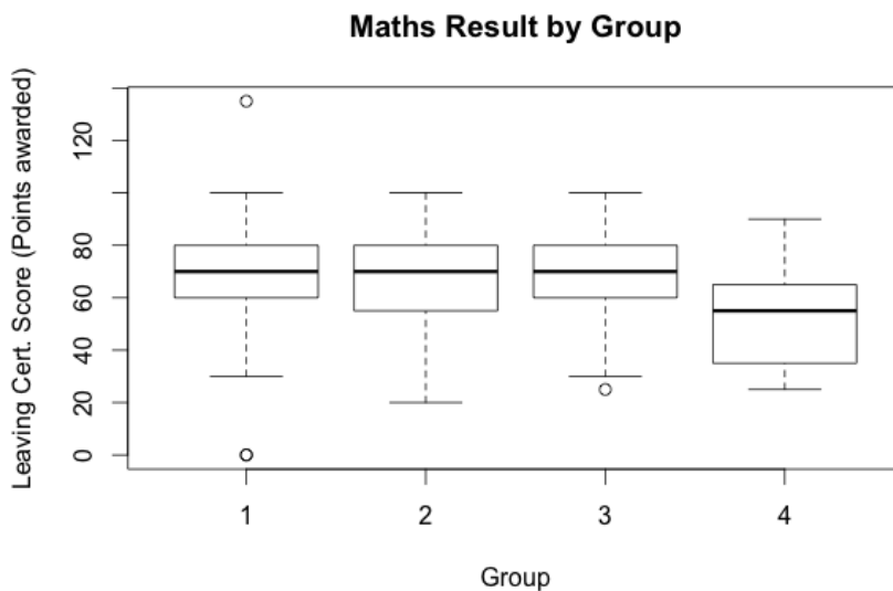
Figure 8: Boxplot of Leaving Cert. mathematics results (in terms of points awarded) by cluster.
