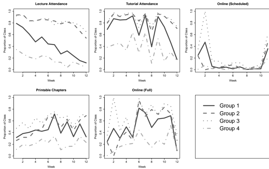
Figure 5: Proportion of clusters attending lectures and tutorials, or engaging with online materials, by week.
