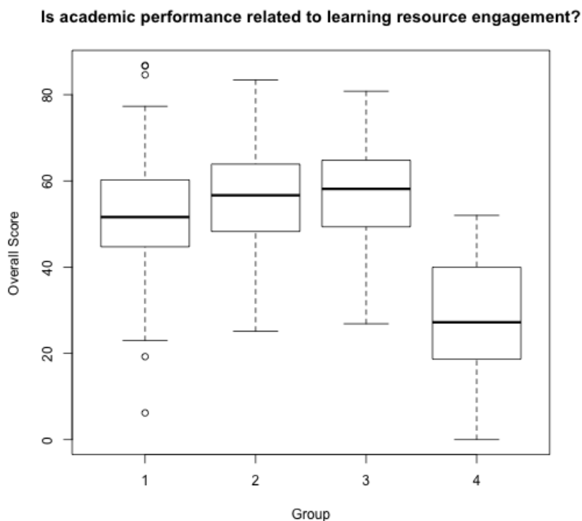
Figure 6: Final score for students by cluster.
