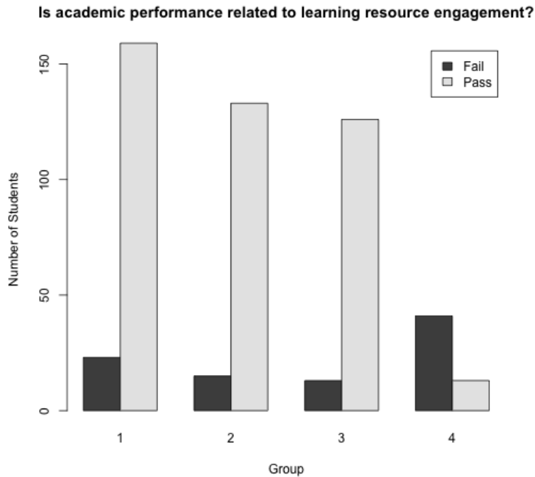
Figure 7: Number of students who passed or failed this module, by cluster.
