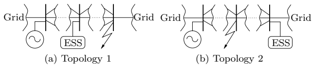
Fig. 2: Topologies of a power system facing a fault: (a) Topology 1: The ESS and the synchronous machines are on the same side with respect to the fault; (b) Topology 2: The fault occurs between the synchronous machine and the ESS.
