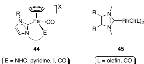
Fig. 11 Redox-active \text{Fe}^{\text{II}} -NHC complexes 44 with metal-carbon \pi interactions and rhodium complex 45 featuring \text{p} acceptor ligands that respond on modifications of substituents \text{R} .
