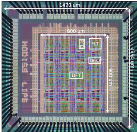
FIGURE 3: Die microphotograph of the distributed clock generator with 4 \times 4 digitally controlled oscillators designed and manufactured in 65 nm CMOS technology.
