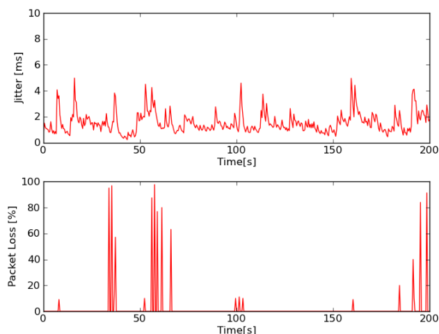
Figure 6. Emergency VoIP call performance in a wireless mesh network
