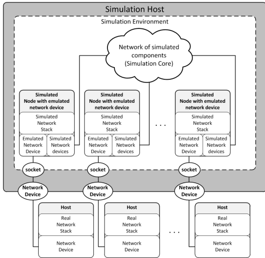
Figure 2. The diagram of the network emulation concept
