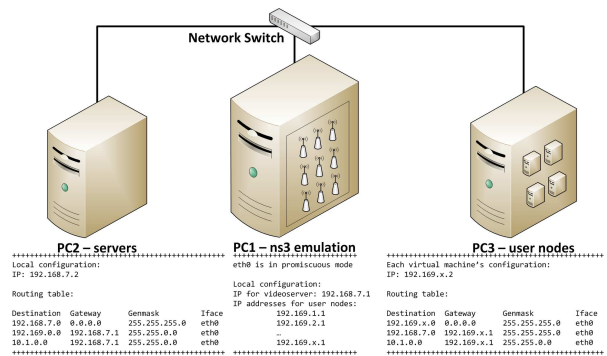
Figure 3. Emulation Setup
