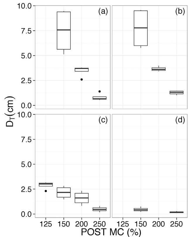
Fig. 5. Observations of spread distance ( D_T ) into POST peat. Subplots are for PRE peats of (a) 25%, (b) 50%, (c) 100% and (d) 125% MC.
