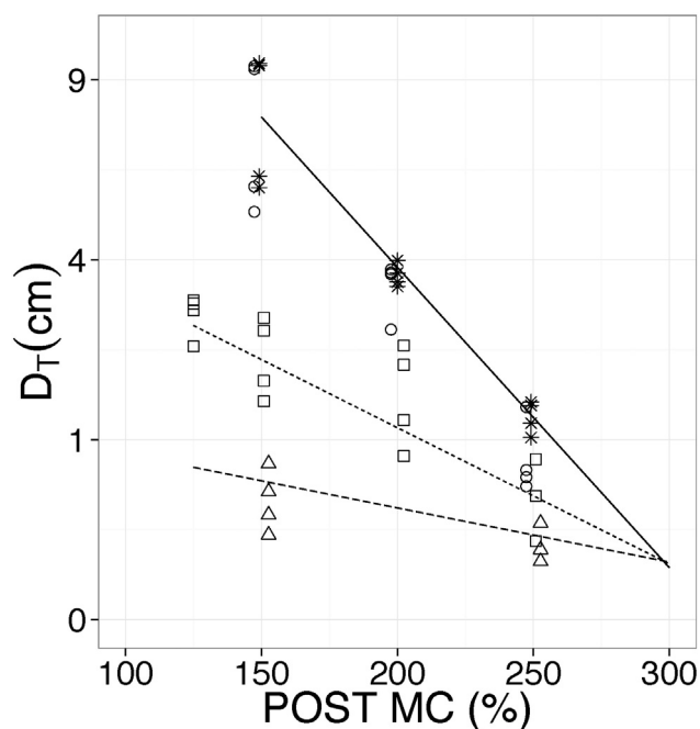
Fig. 6. Spread distance ( D_T ) as function of POST moisture gradient. Symbols represent experimental observations for PRE conditions, circle = 25%, star = 50%, square = 100%, triangle = 125% MC . Lines are model predictions from the coefficients in Table 3.
