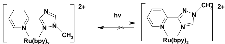
Figure 9 Photo induced irreversible N2 to N4 isomerisation for [\text{Ru}(\text{bpy})_2(1\text{Mepytr})]^{2+}
