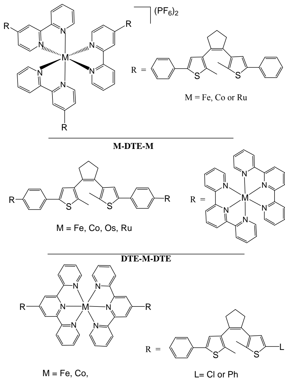
Figure 29 Dithienylethene complexes
