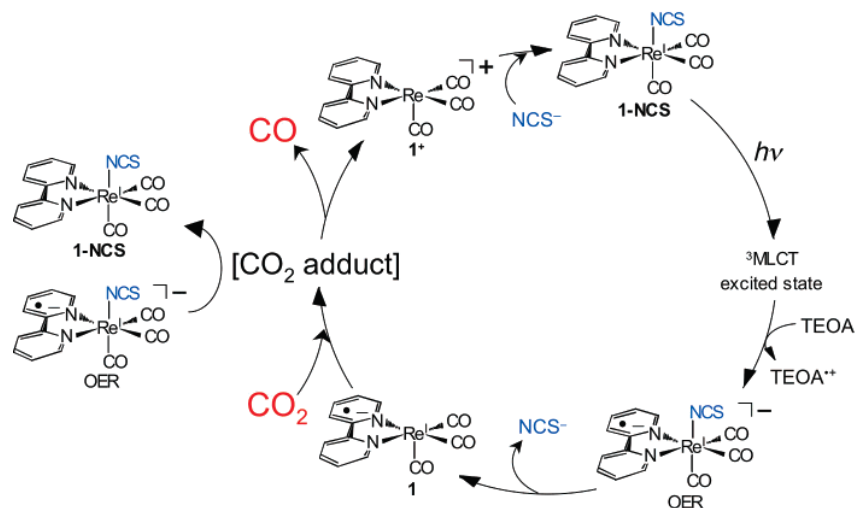
Figure 4 Reaction mechanism for photocatalytic reduction of \text{CO}_2 to \text{CO} using \text{fac-}[\text{Re}(\text{bpy})(\text{CO})_3\text{NCS}] as photocatalyst. Reproduced from ref [19a] with permission of the American Chemical Society.
