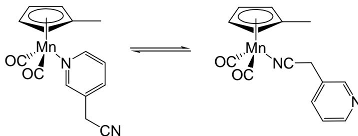
Figure 16 Linkage isomerisation in (\eta^5-C_5H_4CH_3)(CO)_2L type complexes (where L= 3-cyanomethylpyridine)
