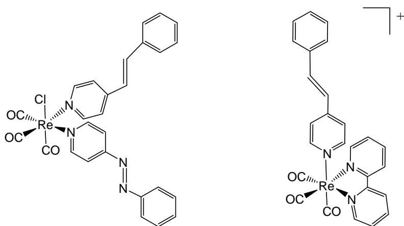
Figure 22. Structures of fac-[ReCl(CO)_3(stpy)_2] and fac-[Re(stpy)(CO)_3(bpy)]^+
