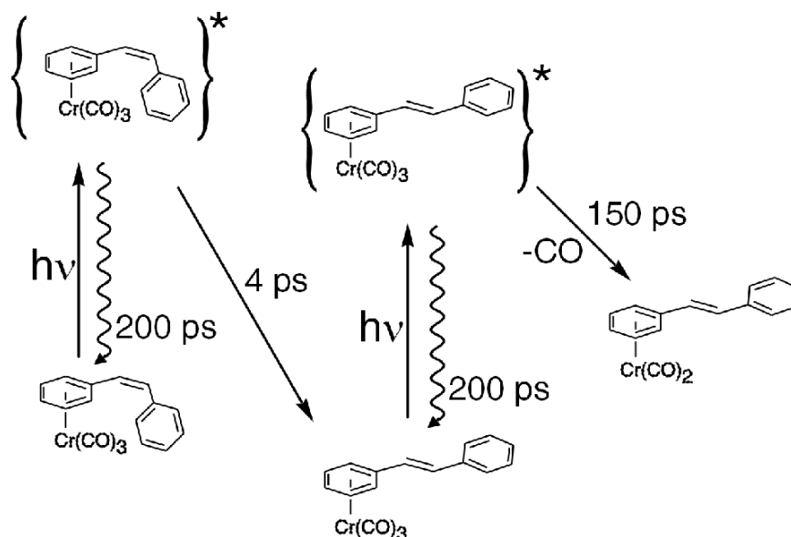
Figure 24. Various intermediates and photoproducts observed following irradiation of cis and trans ( \eta^6 -stilbene)Cr(CO) 3 .
