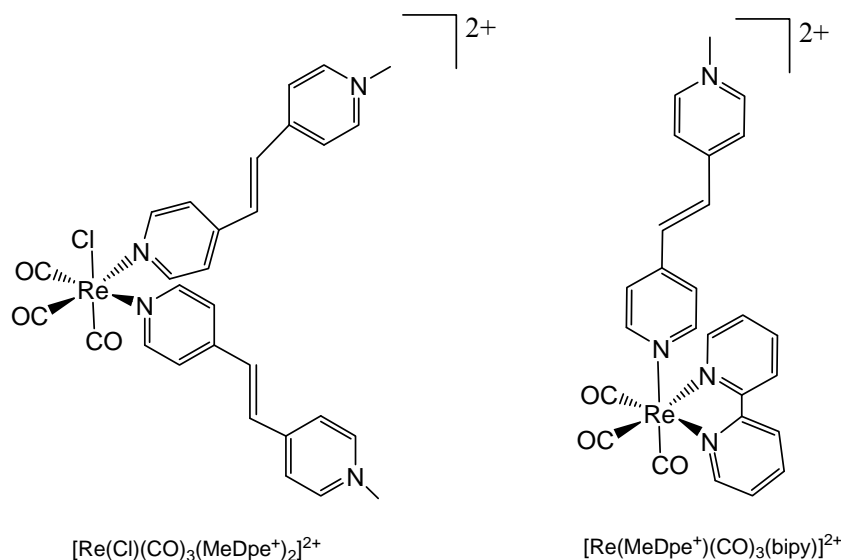
Figure 19 [\text{Re}(\text{Cl})(\text{CO})_3(\text{MeDpe}^+)_2]^{2+} and [\text{Re}(\text{MeDpe}^+)(\text{CO})_3(\text{bpy})]^{2+}
