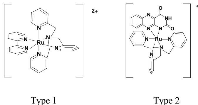
Figure 14 TPA based metal complexes
