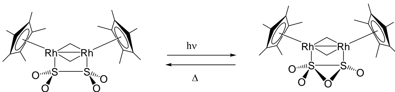
Figure 30. Structures for [(RhCp^*)_2(\mu-CH_2)_2(\mu-O_2SSO_2)] and [(RhCp^*)_2(\mu-CH_2)_2(\mu-O_2SOSO)] .
