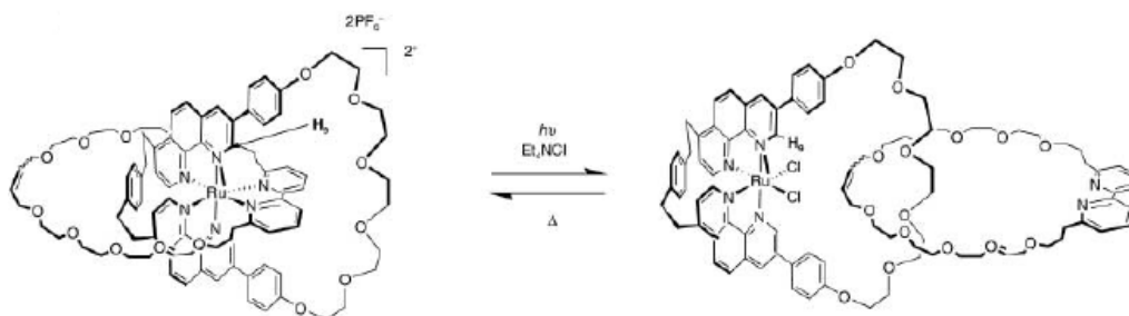
Figure 2 Photochemical and thermal rearrangement for a ruthenium catenane complex. Reproduced with permission by the Royal Society of Chemistry from reference [34].
