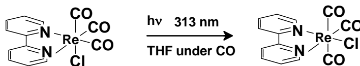
Figure 7 fac - to mer - isomerisation for fac -[Re(bpy)(CO) 3 Cl].
