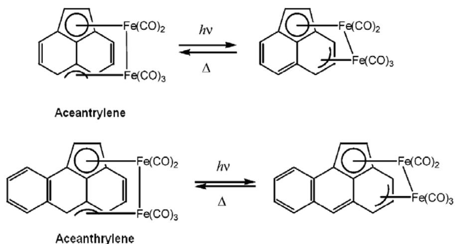
Figure 27 (\mu^2, \eta^3: \eta^5\text{-acenaphthylene})\text{Fe}_2(\text{CO})_5 and (\mu^2, \eta^3: \eta^5\text{-aceanthrylene})\text{Fe}_2(\text{CO})_5
