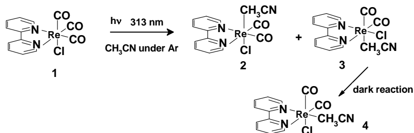
Figure 5. Photoinduced and thermal processes observed upon irradiation of fac -[Re(bpy)(CO) 3 Cl] at 313 nm
