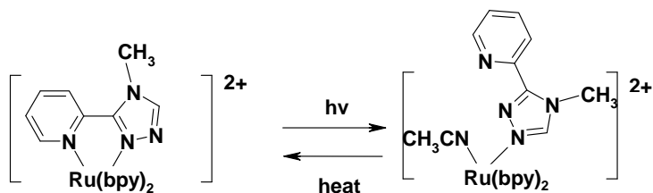
Figure 11 Reversible photochemical/thermal linkage isomerisation for [\text{Ru}(\text{bpy})_2(4\text{Mepytr})]^{2+} .
