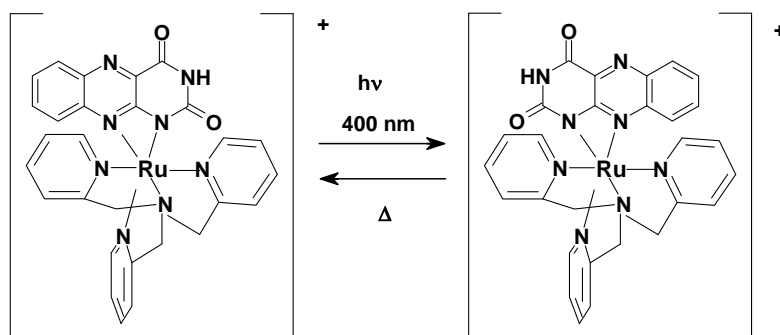
Figure 15 Reversibly photochemical/thermal ligand rearrangements
