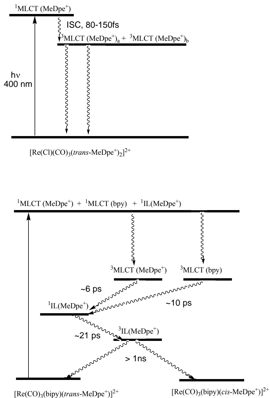
Fig 20. Proposed mechanism for deactivation for both [\text{Re(Cl)(CO)}_3(\text{MeDpe}^+)_2]^{2+} and [\text{Re(MeDpe}^+)(\text{CO)}_3(\text{bipy})]^{2+} . The subscripts a and b denote two ^3\text{MLCT} states of similar origin.
