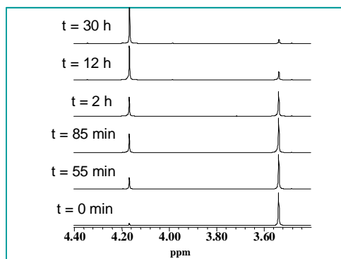
Figure 10 ^1\text{H} NMR spectra taken during photolysis of N2 to N4 isomer in d_6 -acetone. Reproduced with permission from Wiley Publishers from reference [47].
