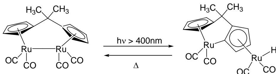
Figure 28. The \text{CMe}_2 bridged dicyclopentadienyl diruthenium complex [\text{Me}_2\text{C}(\eta^5\text{-C}_5\text{H}_4)_2\text{Ru}_2(\text{CO})_4]
