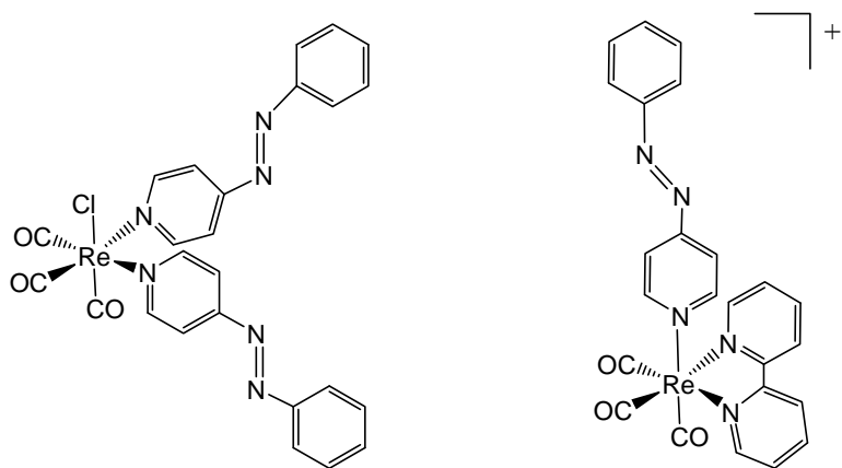
Figure 21 Structures of \text{fac-}[\text{Re}(\text{Cl})(\text{CO})_3(\text{papy})_2] and \text{fac-}[\text{Re}(\text{papy})(\text{CO})_3(\text{bpy})]^+
