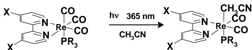
Figure 3 Photoinduced CO loss upon irradiation at 365 nm of fac - [\text{Re}(\text{X}_2\text{bpy})(\text{CO})_3(\text{PR}_3)]^+
