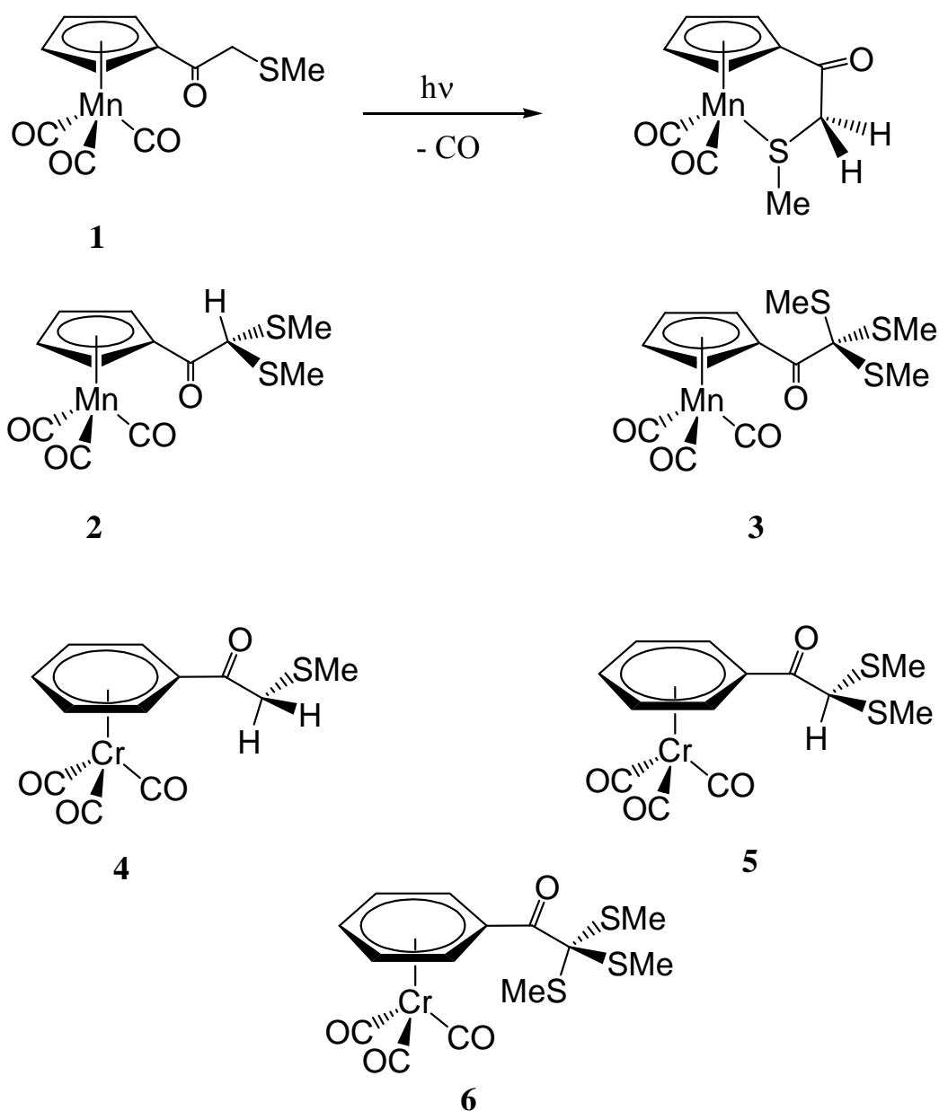
Figure.17. Cyclopentadienyl \text{Mn}(\text{CO})_3 and Arene chromium tricarbonyl derivatives with mono, di and tri-pendant sulphides
