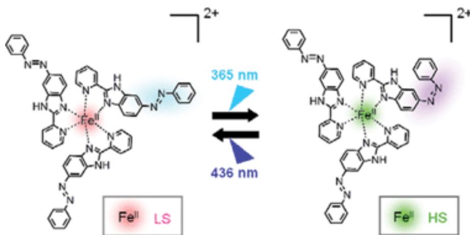
Figure 23. Light-driven spin change for by isomerisation of azobenzene containing ligand. Reproduced from Ref 62 with Permission of the Royal Society of Chemistry.
