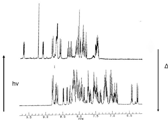
Figure 12 ^1\text{H} NMR spectra illustrating the photochemical/thermal rearrangements shown in Figure 11.
