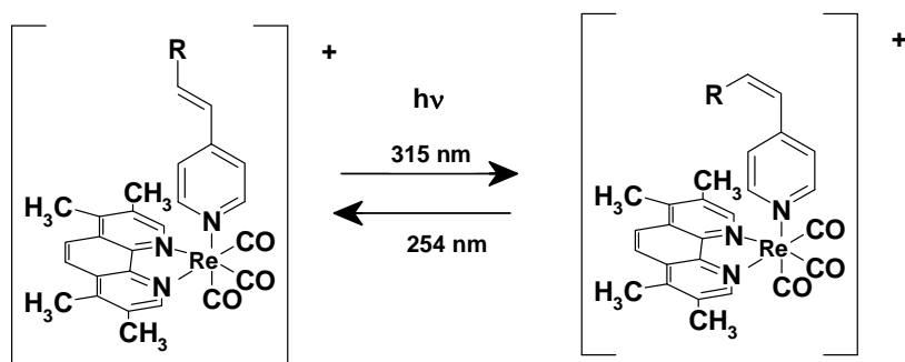
Figure 18. Trans - cis isomerisation of stpy type ligand in fac -[Re(Me 4 phen)(CO) 3 (stpy)] +
