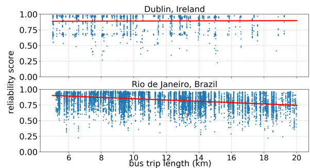
Fig. 3. Reliability score v.s. bus trip length
