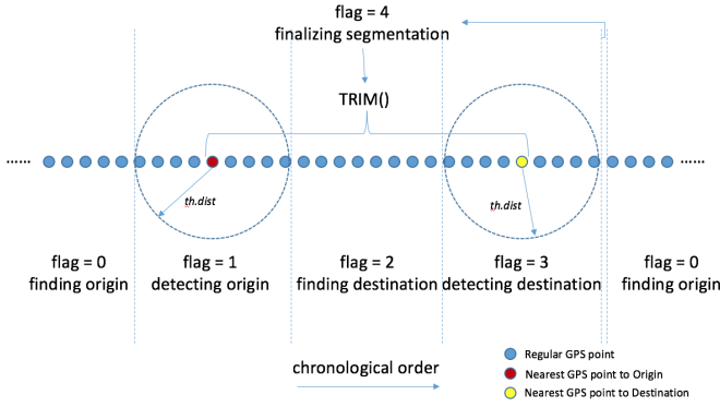
Fig. 2. Diagram of trip segmentation algorithm
