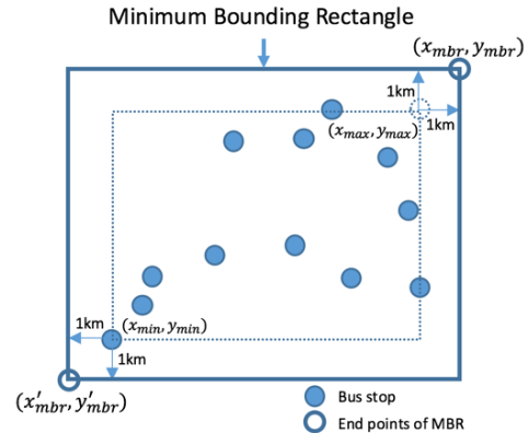
Fig. 1. Minimum bounding rectangle used to filter GPS outliers
