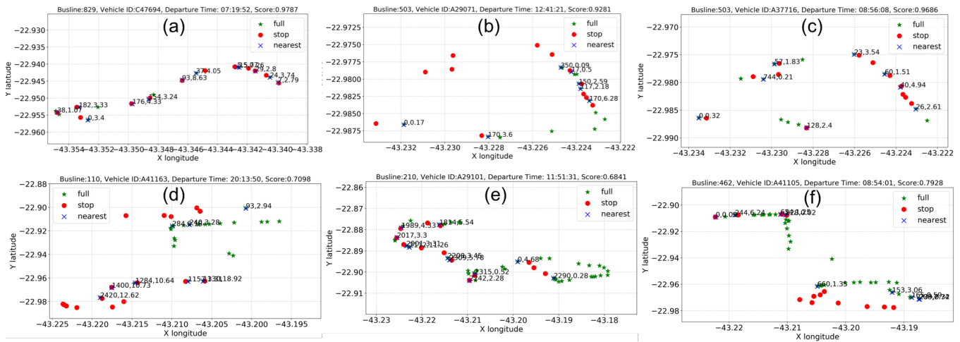
Fig. 4. Bus trajectory comparison in Rio. (“star” represents full bus trajectory points; “circle” represents predefined bus stops; “cross” represents the nearest bus trajectory points (subset of “star”) to each of its predefined bus stops, it also displays “time_deviation(seconds), speed(m/s)”) )
