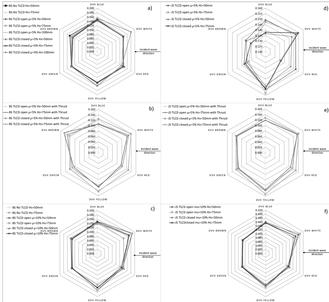
Figure 3: DVV analysis results (RMSE) for waves with T_p=2.4s and f_p=0.42Hz a-c) Bretschneider spectra: a) for H_{s,m}= 50, 75, and 100mm without TLCD and with open and closed TLCD ( \mu=5\% ); b) for H_{s,m}= 50 and 75mm with open and closed TLCD ( \mu=5\% ), and with thrust loading; c) for H_{s,m}= 50, and 75mm without TLCD and with open and closed TLCD ( \mu=10\% ), and d-f) JONSWAP spectra: d) for H_{s,m}= 50 and 75mm with open and closed TLCD ( \mu=5\% ); e) for H_{s,m}= 50 and 75mm with open and closed TLCD ( \mu=5\% ), and with thrust loading; f) for H_{s,m}= 50, and 75mm with open and closed TLCD ( \mu=10\% ).
