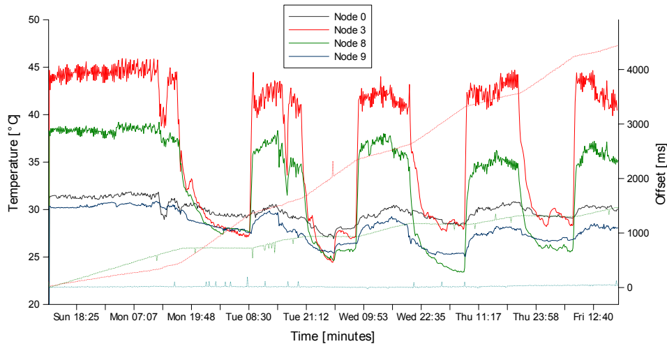
Fig. 16: Clock drift change caused by temperature
