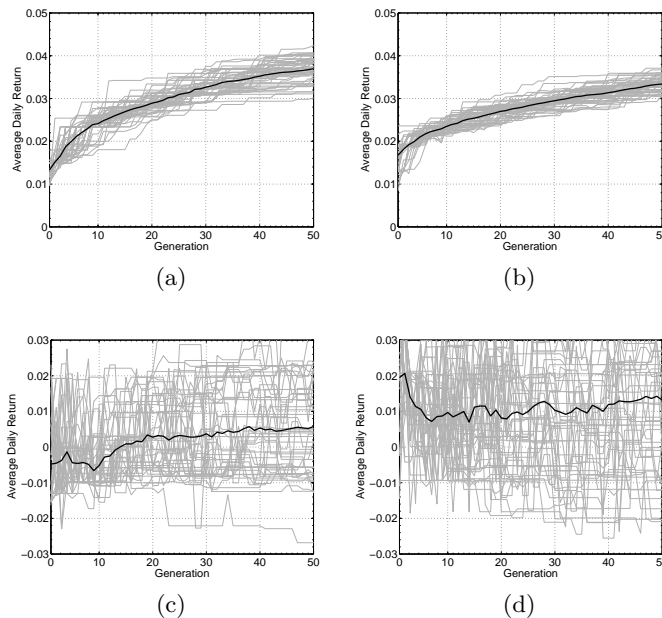
Fig. 1. Evolution of best-of-generation average daily return. (a) and (b) show in-sample evolution using sets of weighting coefficients represented by the tuples (1.0, 0.0) and (0.2, 0.8) respectively; (c) and (d) show the out-of-sample evolution for the same weighting coefficient setups. Each graph presents 50 evolutionary runs; average in bold.
