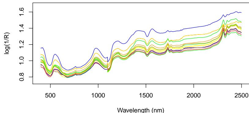
FIG 1. The near-infrared spectra recorded for three examples of each meat species in the study. The discontinuity at 1100 nm is due to a sensor change at that value. The samples are colored as Beef=red, Lamb=green, Pork=blue, Turkey=orange, Chicken=yellow.
