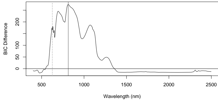
FIG 5. A plot of the BIC difference for each wavelength given that wavelength 626 nm is already accepted. The wavelength with the greatest BIC difference is 814 nm. Note that wavelengths close to 626 nm still have positive BIC difference values.
