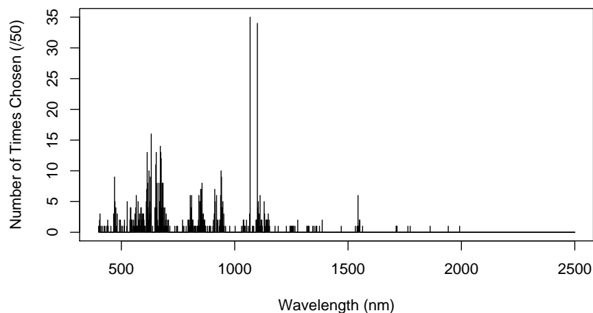
FIG 7. Wavelengths chosen in the five meat classification problem for the variable selection and updating method. The height of the bars shows how many times the wavelength was chosen in 50 random splits of the data.
