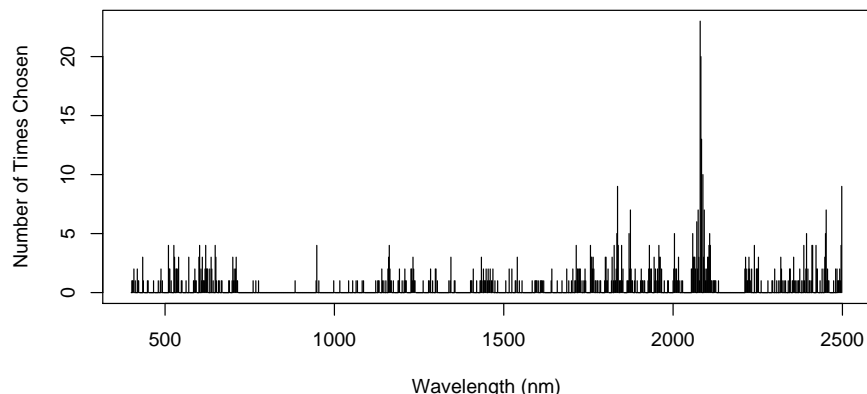
FIG 9. Wavelengths chosen in the olive oil classification problem using variable selection and updating method. The height of the bars shows how many times the wavelength was chosen in 50 random splits of the data.
