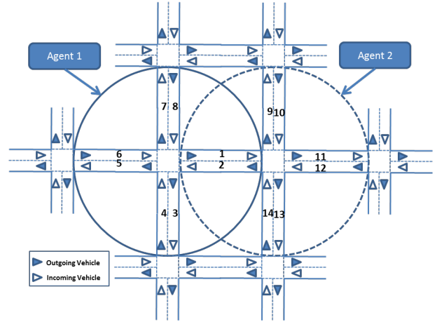
Fig. 5: MAS Design in NRR
