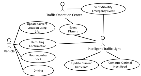
Fig. 4: Use case diagram of all key actors in NRR
