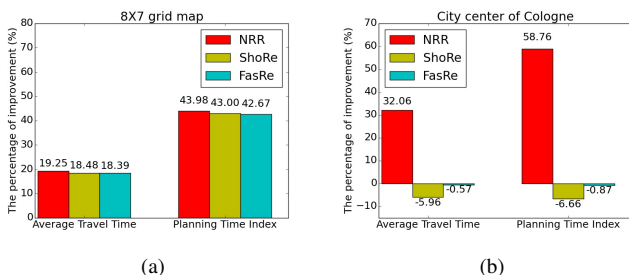
Fig. 9: Comparison of the percentage of improvement achieved by NRR, ShoRe and FasRe over ERE in terms of ATT and PTI
