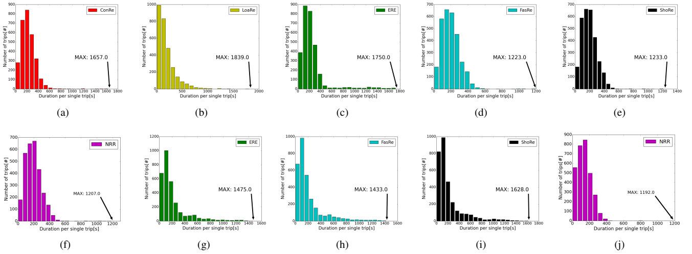
Fig. 8: Trip duration distribution of the evaluated scenarios in both 8X7 grid map (a-f) and city center of Cologne (g-j)
