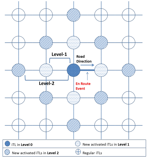
Fig. 3: Activated iTTLs in different NRR levels
