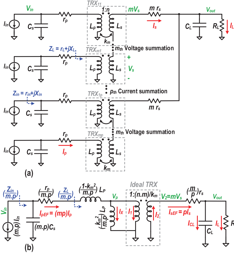
Fig. 14. (a) Transformer-based matching network with m -way voltage and p -way current summation; and (b) its equivalent circuit model.
