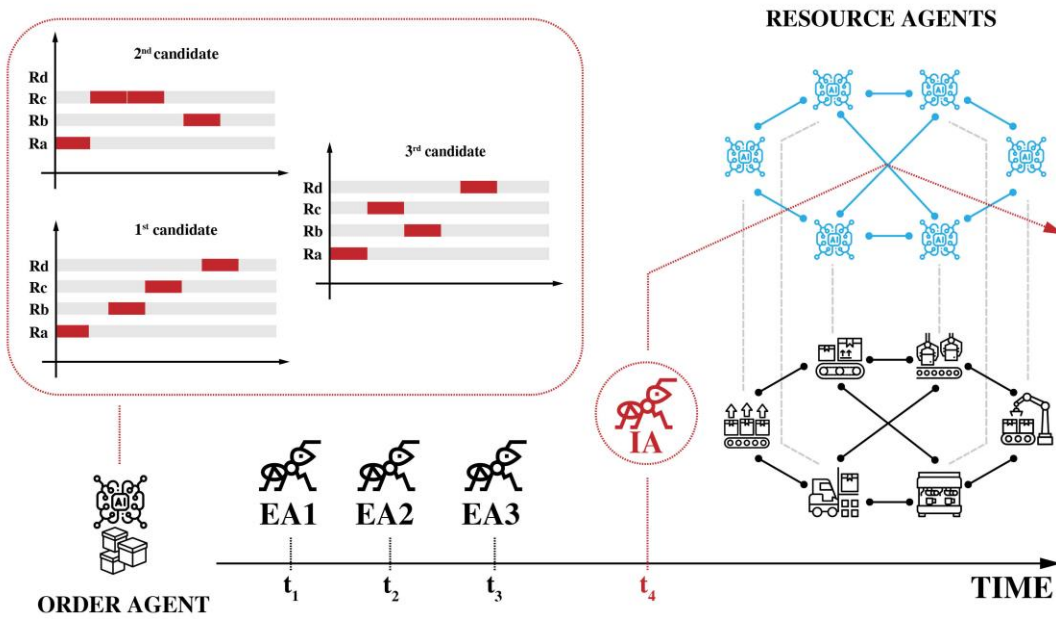
Figure 17: Ant agents scout for solutions on behalf of their order agent in a manufacturing execution system (EA: exploring ant, IA: intention ant) adapted from [Valckenaers et al., 2005].
