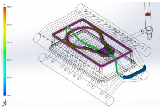
Figure 24: Optimised coolant channels of an injection moulding die, based on the dicot leaves structure, produced by AM [Carson, 2015].
