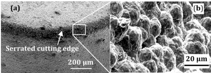
Figure 13: Biomimetic tools: (a) cutting edge with serrated ‘tips’; (b) an assembly of the tips forming the surface features of a lotus leaf and showing the periodicity of the micron tips [Jiang, 2014].
