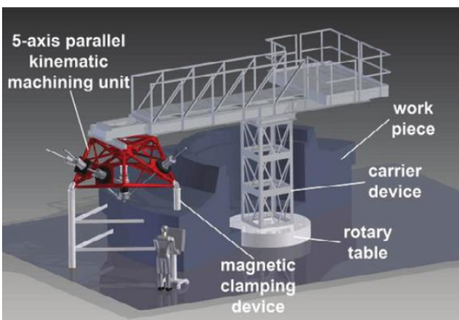
Figure 15: Modular mobile 5-axis parallel kinematic machine tool [Neugebauer et al., 2012].
