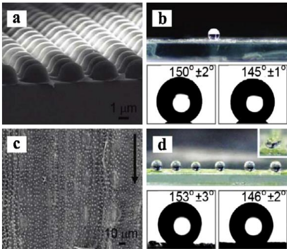
Figure 7: Artificial surface inspired by rice leaf providing both super-hydrophobicity and anisotropic wettability [Xia et al., 2012].
