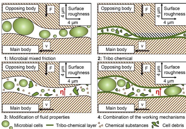
Figure 14: Possible working mechanisms of the microbial-based metalworking fluid [Meyer et al., 2017].
