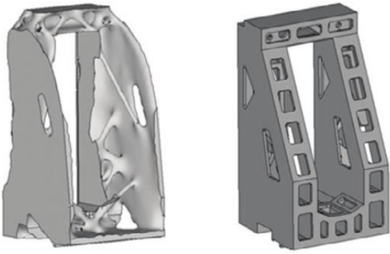
Figure 16: Topological optimisation of a machine stand (left) and the technical interpretation (right) [Neugebauer et al., 2012].
