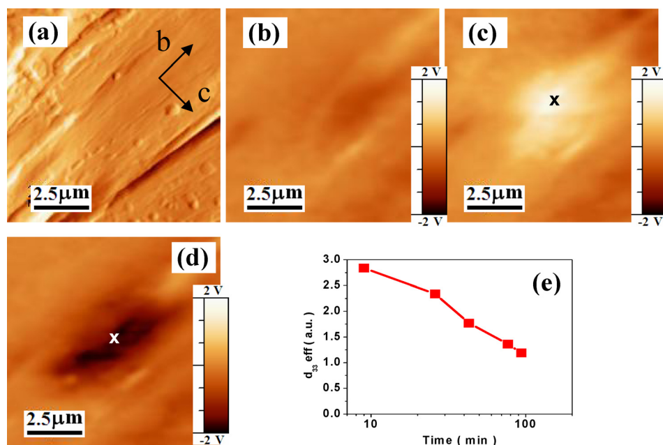
FIG. 7. (a) Topography (deflection) image of a thymine crystal ( 1.0\ \text{mg ml}^{-1} concentration). PFM images: (b) before poling, (c) after poling + 100 V for 10 s, (d) after -100 V for 10 s. (x shows the position of poling with the cantilever). (e) Time relaxation of the PFM signal after poling + 100 V for 10 s.
