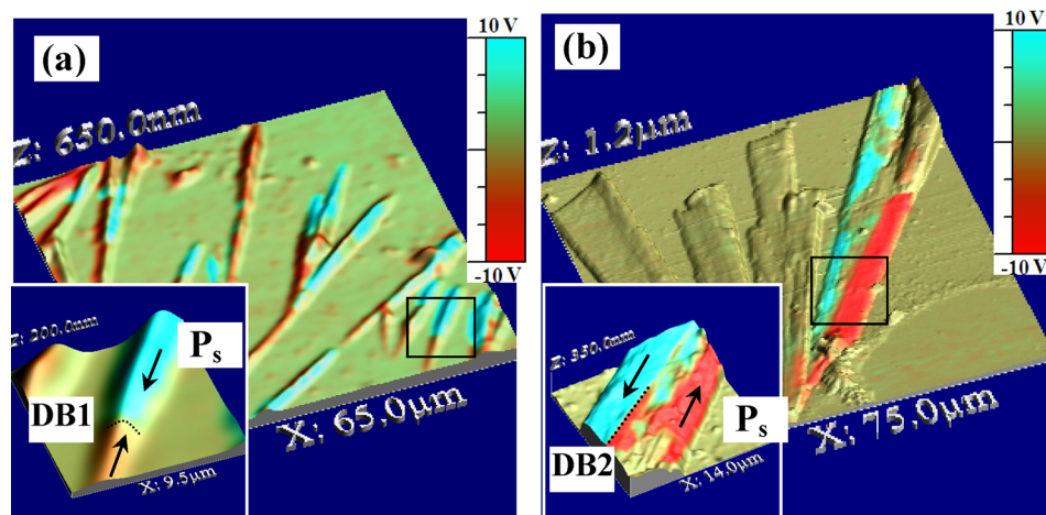
FIG. 4. 3D topography with IP PFM images: (a) needle-like crystals ( 0.1 \text{ mg ml}^{-1} concentration), (b) flat crystals ( 1.0 \text{ mg ml}^{-1} concentration). DB1—head-to-head boundary for the domains, DB2— 180^\circ domain boundary. P_s —domain polarization.
