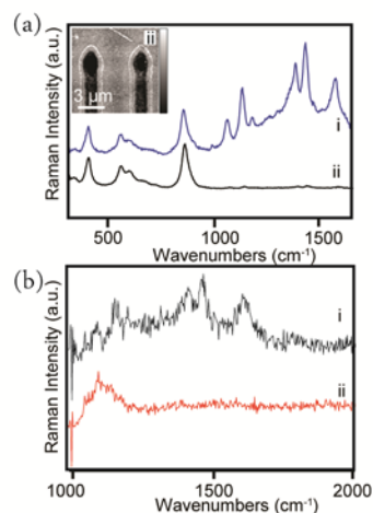
Figure 5. (a) SERS signal from the substrate and the probe molecule 4-aminothiophenol adsorbed onto the Ag nanowires formed on the surface of (i) the periodically proton exchanged area (Figure 4a) and (ii) the region that has been uniformly proton exchanged with periodic RIE stripes (AFM topography image is shown as an inset to (a)). (b) (i) SERS signal from the same region as a(ii), and (ii) the signal from 4-aminothiophenol and LN for a sample exposed to the 4-aminothiophenol-methanol solution after the nanowires have been removed (for wavenumbers greater than 1000). The z -data scale for the inset in (a) is 10 nm.
