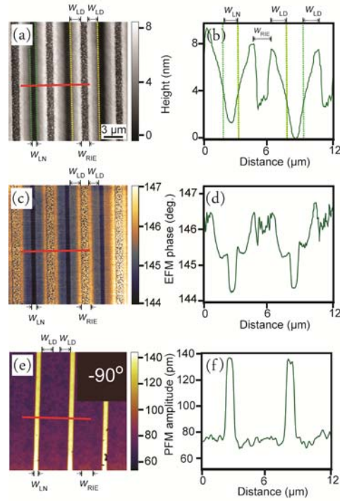
Figure 3. +z PPELN surface prior to photodeposition. (a) AFM topography image, and (b) the corresponding line profile from the region indicated in (a). (c) EFM phase image, and (d) the corresponding line profile from the region indicated in (c). (e) PFM amplitude image with an inset of the PFM phase image with a scan area of 20 μm and a data scale of 360°, and (f) the corresponding line profile from the region indicated in (e). The scale bar in (a) also applies to (c, e).
