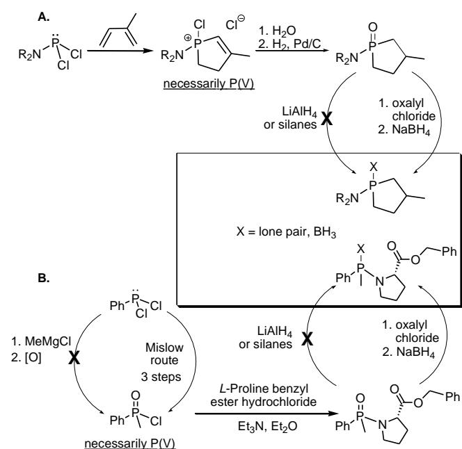
Scheme 2. Examples of aminophosphine boranes difficult to synthesise by other means
