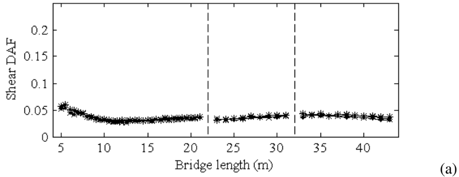
Figure 17: Standard deviation of DAF due to fleet of cranes on class 'A' profile; No damage (•-•-•-•-); 2cm bump depth (x-x-x-x-), 4cm bump depth (*-*-*-*); a) Shear force at 1 st support; b) Bending moment; c) Shear force at 2 nd support
