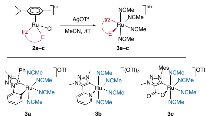
Scheme 2 Synthesis of complexes 3a–c .
