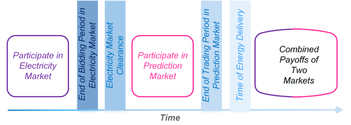
Fig. 1. Schematic representation of combined trading in the electricity market and prediction market over time.
