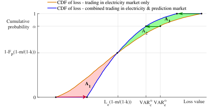
Fig. 3. Effect of trading in prediction market on the probability distribution of the WPP loss.
