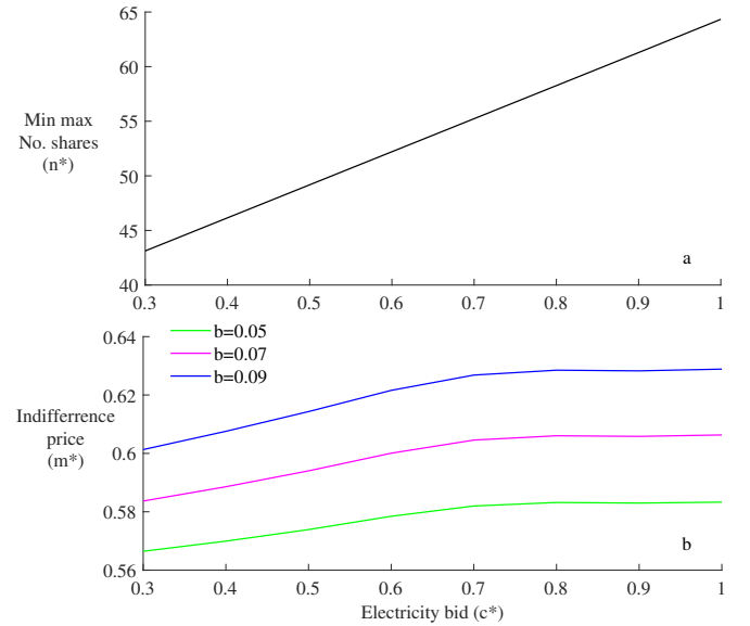
Fig. 8. Effect of electrical bid and risk-aversion on the prediction market trading strategies a) number of shares in min max strategy b) price in utility indifference strategy
