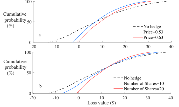
Fig. 7. Comparing the CDF of hedged loss by trading in prediction market against unhedged case: a) the effect of price and b) the effect of number of shares.
