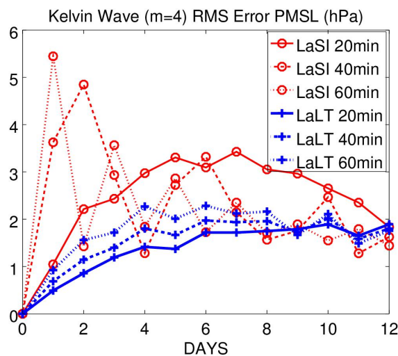
Figure 3. RMS errors for six integrations of Kelvin waves with m = 4 . Red: LaSI scheme. Blue: LaLT scheme.
