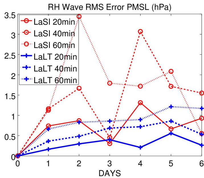
Figure 6. Rossby-Haurwitz wave RH(4,5). RMS errors of surface pressure (hPa) for 6 day forecasts.
