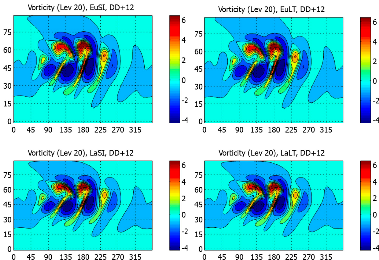
Figure 1. Vorticity field at model level 20 for 12-day forecasts with four integration schemes. Top left: EuSI. Top right: EuLT. Bottom left: LaSI. Bottom right: LaLT. All runs had time step 5 min. Units 10^{-5}\text{s}^{-1} .
