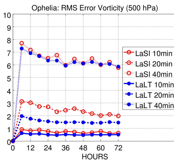
Figure 11. Real data: rms error for 500 hPa vorticity (units 10^{-6}s^{-1} ) over 3 days for LaSI forecasts (red) and LaLT forecasts (blue) with time steps 10, 20 and 40 min.
