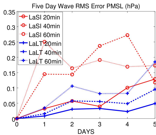
Figure 4. Five-day wave RO(1,2). RMS errors of surface pressure (hPa) for 5 day forecasts.
