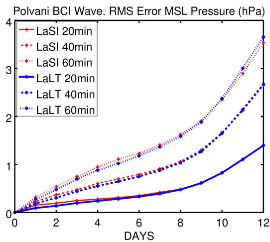
Figure 9. RMS errors in surface pressure for baroclinic wave (Polvani et al. [20]). Red lines: LaSI. Blue lines: LaLT.
