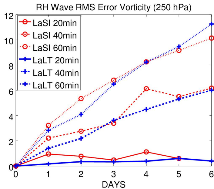
Figure 7. Rossby-Haurwitz wave RH(4,5). RMS errors of 250 hPa vorticity (units 10^{-6}s^{-1} ) for 6 day forecasts.
