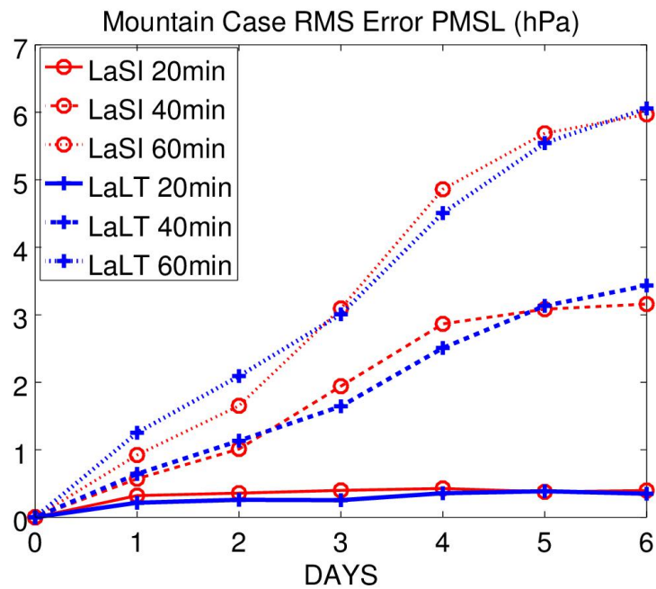
Figure 8. RMS errors in surface pressure for Test Case 5 (Williamson et al. [25]). Red lines: LaSI. Blue lines: LaLT.
