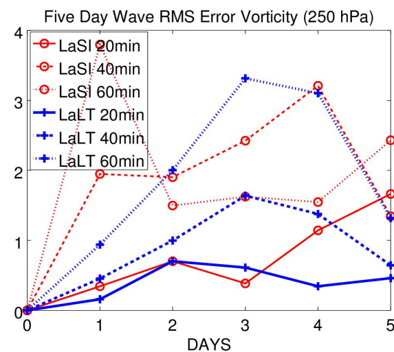
Figure 5. Five-day wave RO(1,2). RMS errors of 250 hPa vorticity (units 10^{-6}s^{-1} ) for 5 day forecasts.
