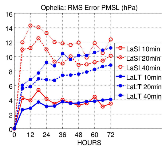
Figure 10. Real data: rms error for surface pressure (hPa) over 3 days for LaSI forecasts (red) and LaLT forecasts (blue) with time steps 10, 20 and 40 min.
