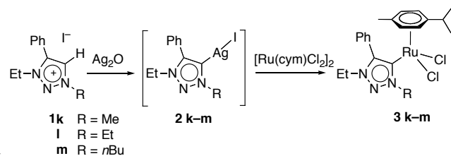
Scheme 2 Synthesis of complexes 3k-m .
