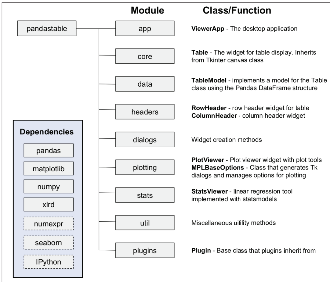
Figure 1: Outline of pandastable library modules. The graphical user interface is a scaffolding using these modules.
