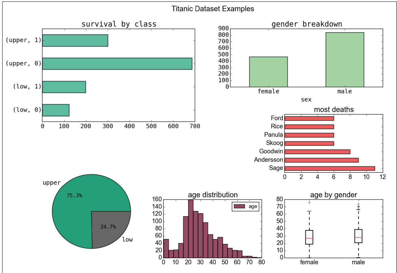
Figure 3: A figure generated directly from the application using the Titanic data. This uses the grid layout mode to combine multiple sub plots together.
