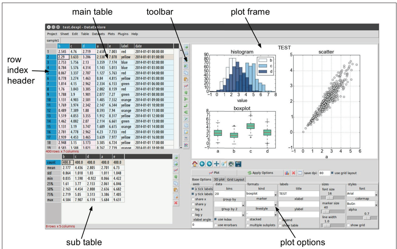
Figure 2: Application interface.
