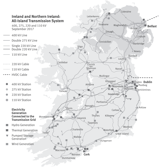
Fig. 4: All-island Irish power system map (available at: www.eirgridgroup.com ).
