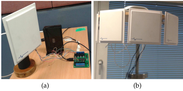
Fig. 4: Directional AP antennas: (a) motorized, (b) multi-antennas.
