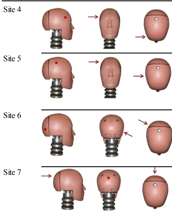
Figure 3. Impact sites on the unhelmeted Hybrid III headform similar to those from standard helmet methods.
