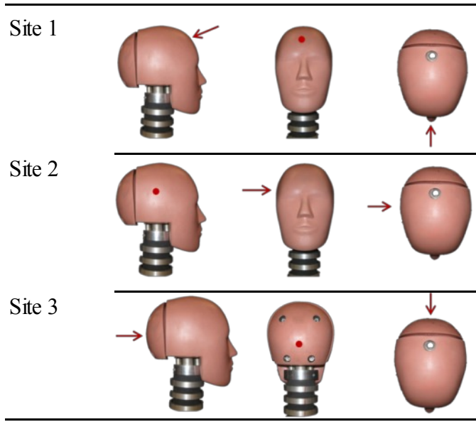
Figure 3. Impact sites on the unhelmeted Hybrid III headform similar to those from standard helmet methods.
