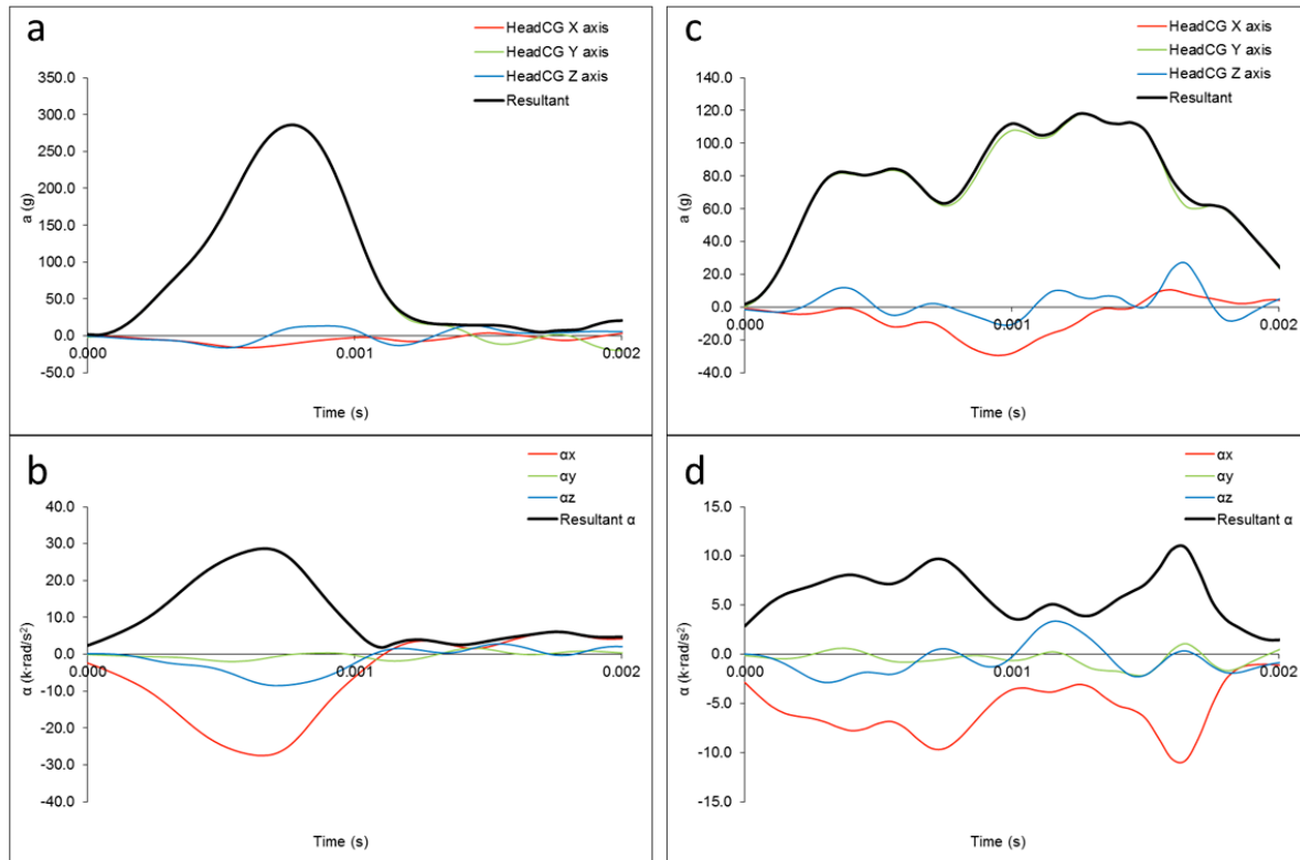
Figure 5. Comparison of the acceleration loading curves for helmet C (a and b) and D (c and d) for the site 2 impact
