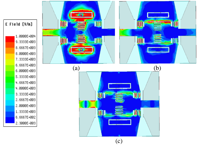
Fig. 6. Electric field distribution in (a) 2.8, (b) 5.2, (c) 9.5GHz
