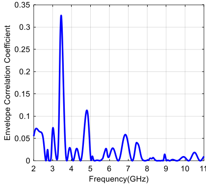
Fig. 7. Calculated Envelope Correlation Coefficient
