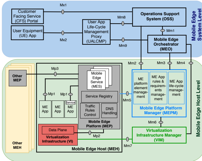
Fig. 3: MEC reference architecture.
