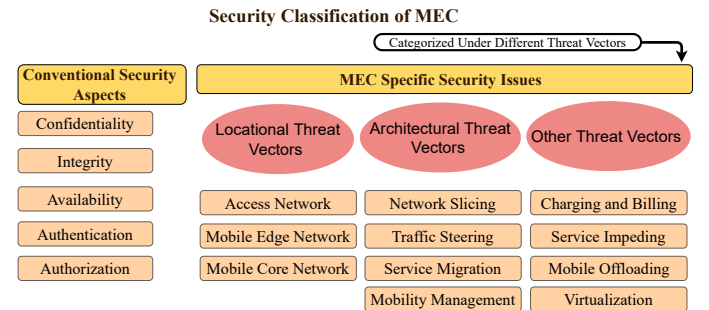
Fig. 2: Classification of MEC security.
