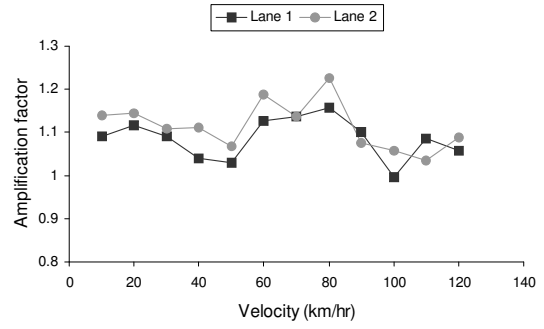
(b) - Three-axle vehicle
