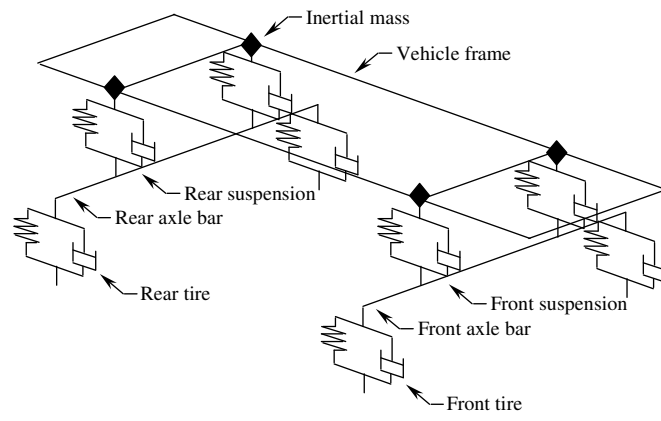
Figure 11 – Generic vehicle model (González , 2001)
