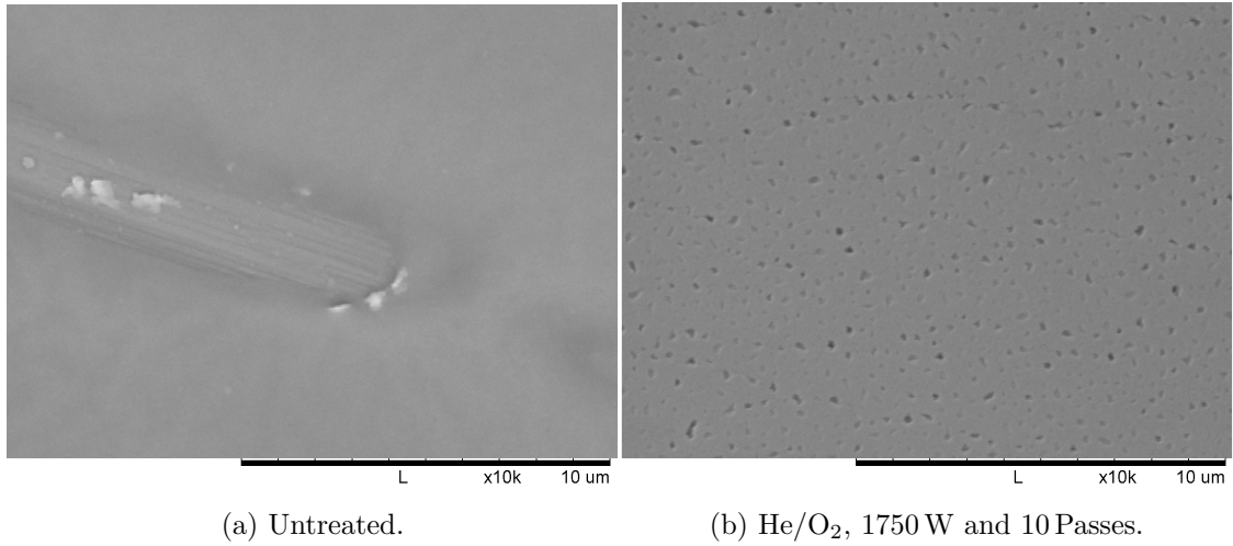
Figure 16: SEM image of the surface of (a) an untreated prepreg and (b) one treated with a He/O 2 plasma at 1750 W for 10 Passes.
