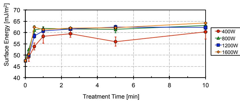
Figure 9: Comparison of total surface energy from Figure 8. Note that in some cases, the error bars are obscured by the data points.
