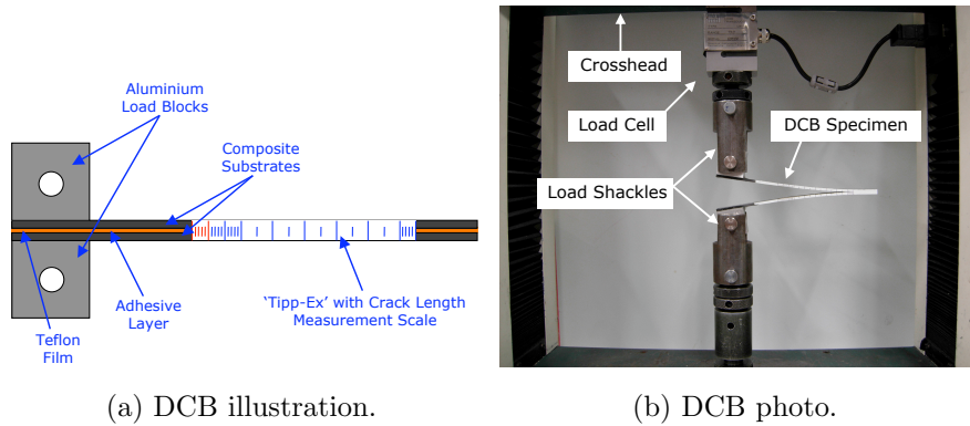
Figure 1: Illustrations and photographs of DCB experimental setup.
