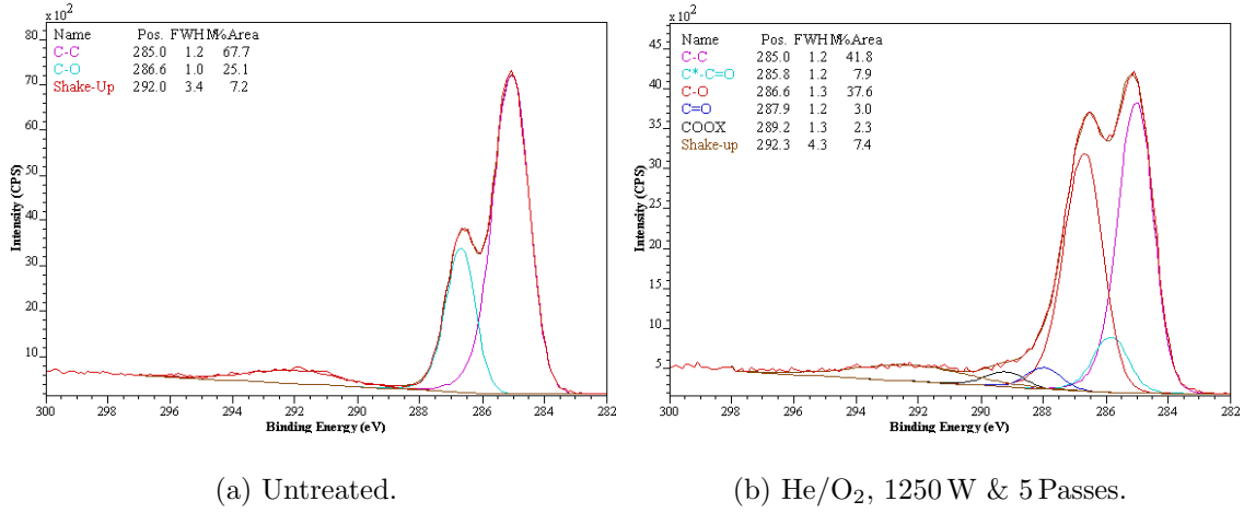
Figure 12: XPS spectra for untreated prepreg and after a He/O 2 plasma treatment.
