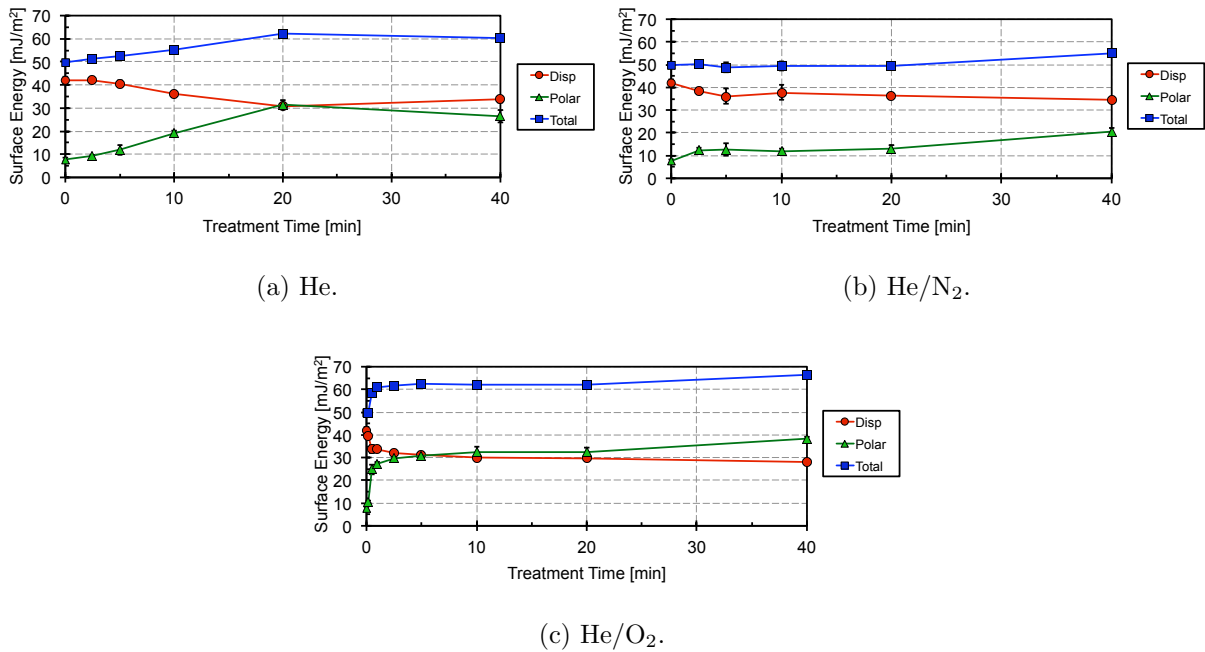
Figure 5: Surface energy results for He, He/N 2 & He/O 2 plasmas at 1200W as a function of treatment time. These readings were taken approximately 2 hours after treatment. Note that in some cases, the error bars are obscured by the data points.
