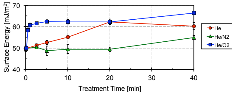
Figure 6: Comparison of total surface energy from Figure 5. Note that in some cases, the error bars are obscured by the data points.
