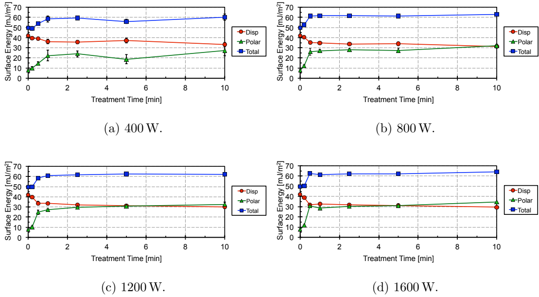
Figure 8: Surface energy results for a He/O 2 plasma at various applied powers and treatment times. Note that in some cases, the error bars are obscured by the data points.
