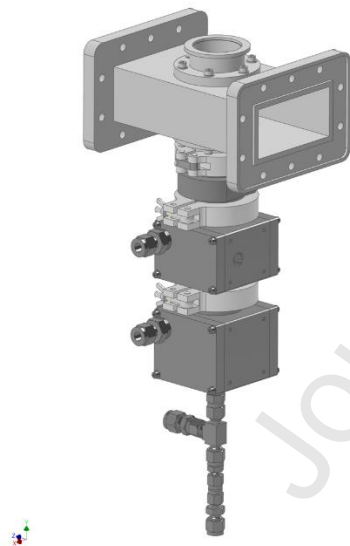
Figure 1: Schematic diagram of the microwave plasma sources PLexc 2 .
