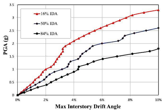
(a) With fully-rigid connection
