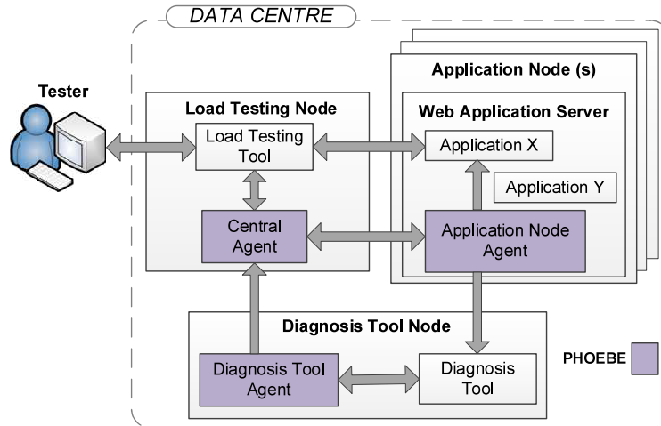
Figure 1. PHOEBE: An Automation Framework for Performance Testing.
