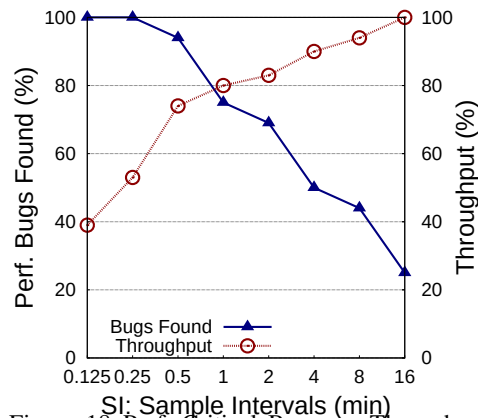
Figure 18. Perf. Critical Bugs vs. Throughput - EMAT.
