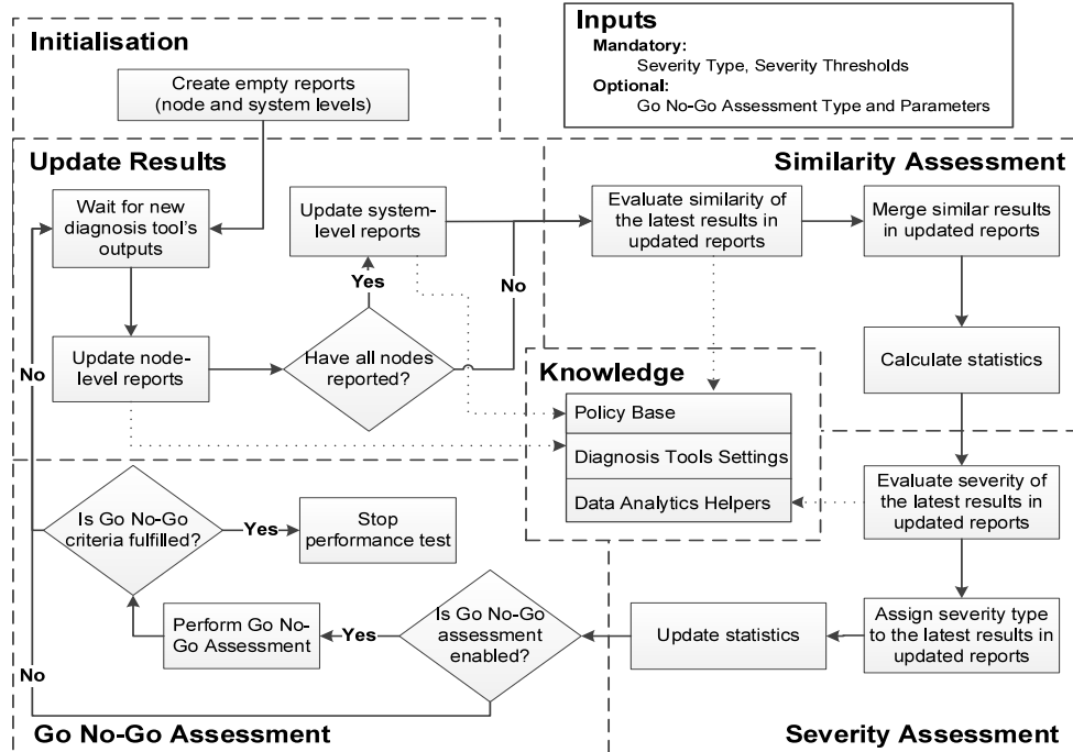
Figure 10. Multi-View Consolidation Policy.
