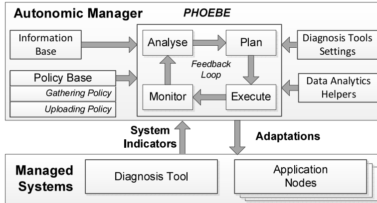
Figure 3. PHOEBE - Conceptual View.
