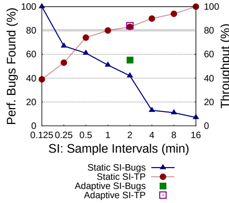
Figure 29. Perf. Bugs vs. Throughput - EMAT.
