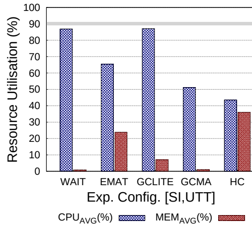
Figure 31. Resources vs. Configuration - All Tools.
