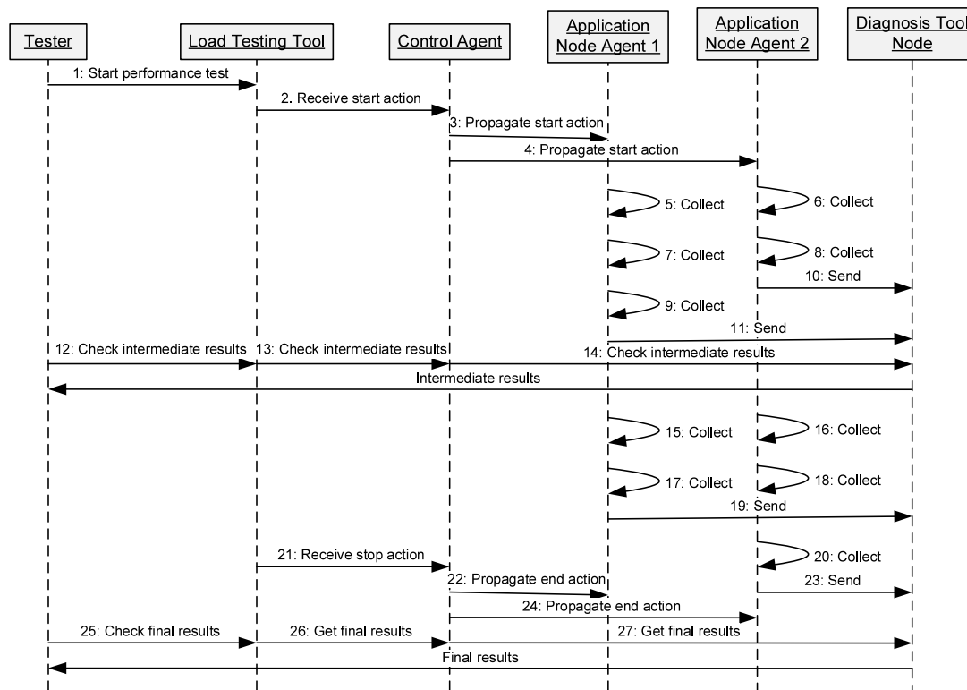
Figure 7. PHOEBE - Sequence diagram.
