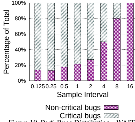
Figure 19. Perf. Bugs Distribution - WAIT.
