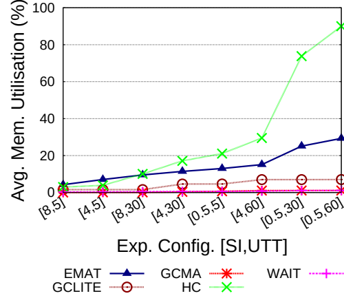
Figure 26. Avg. MEM Utilisations per Tool.
