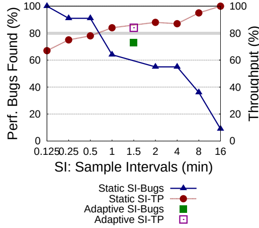
Figure 30. Critical Perf. Bugs vs. Throughput - WAIT.
