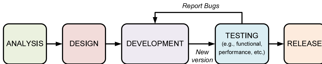
Figure 2. Traditional Software Development Process.
