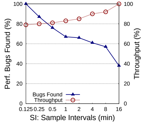
Figure 13. Perf. Bugs vs. Throughput - HC.
