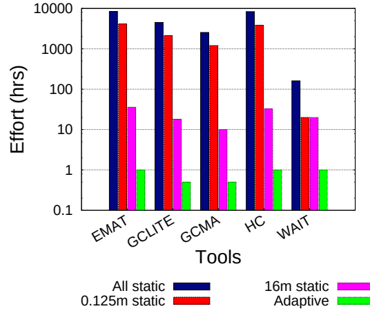
Figure 32. Performance Analysis Effort-savings.
