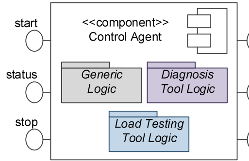
Figure 5. Control Agent - Component Diagram.
