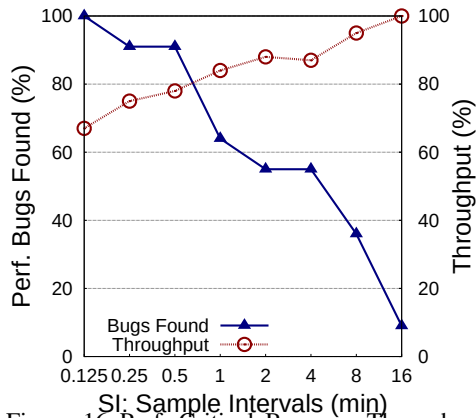
Figure 16. Perf. Critical Bugs vs. Throughput - WAIT.
