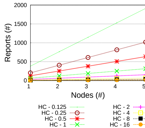
Figure 24. Consolidated Reports per Tool/Hour.
