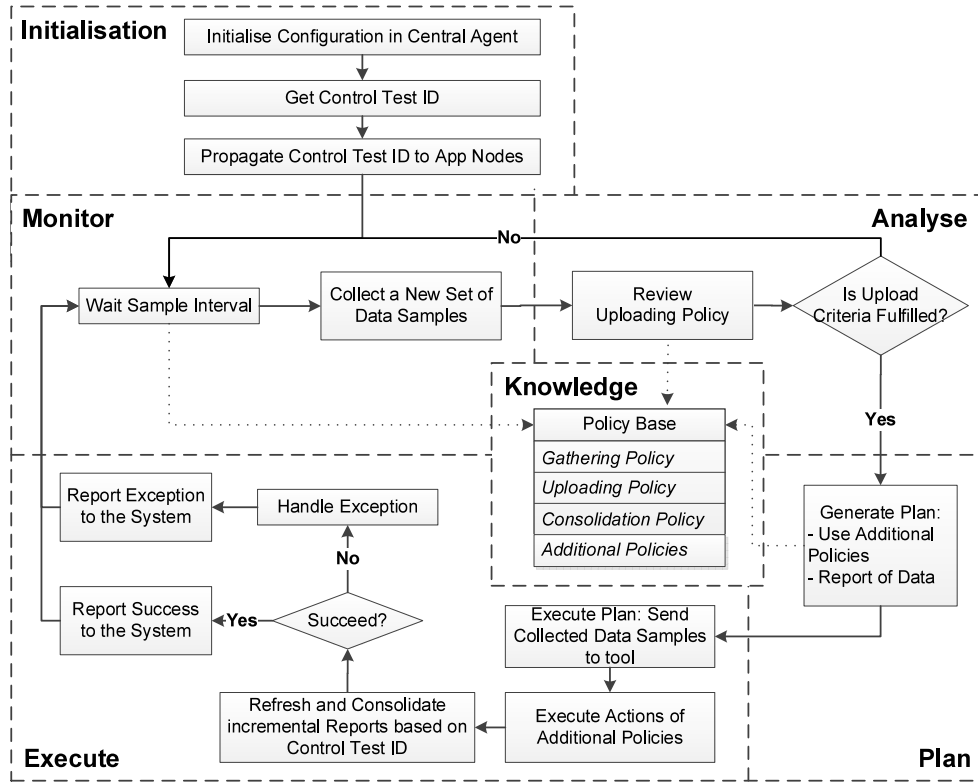
Figure 4. PHOEBE - Core Process.
