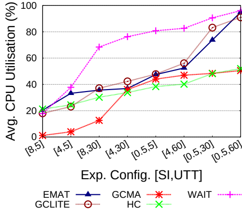
Figure 25. Avg. CPU Utilisations per Tool.
