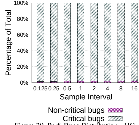
Figure 20. Perf. Bugs Distribution - HC.
