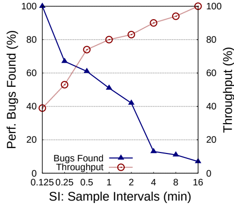
Figure 14. Perf. Bugs vs. Throughput - EMAT.
