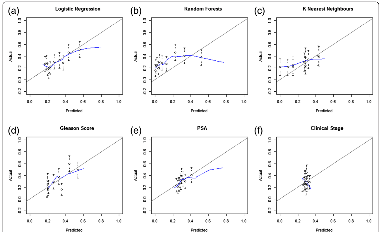
Figure 3 Calibration curves which illustrate predicted probabilities on the x-axis and the actual outcome on the y-axis. In this case the outcome is a binary variable hence Loess smoothing (blue line) was used to estimate the actual outcomes for (a) logistic regression model, (b) random forests model, (c) k nearest neighbours model, (d) biopsy Gleason score, (e) PSA and (f) clinical stage.
