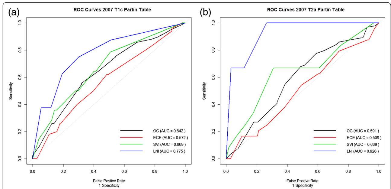
Figure 2 Predictions from the 2007 Partin tables. The patient's data was applied to the 2007 (a) T1c and (b) T2a Partin tables and the discriminate ability measured using ROC curves and AUC values. The AUC values of the ECE predictions are lower than those of the logistic regression model developed in this study.
