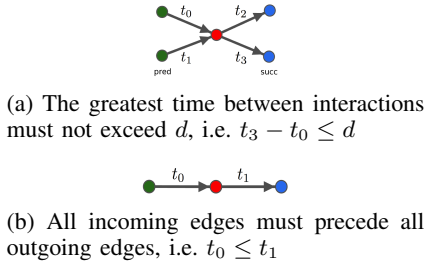
Fig. 1: Semantic feasibility tests, for all nodes in the mapping.
