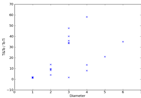
Fig. 2: The ratio of Ti\&To / To-Ti compared with the diameter of each subgraph (jitter applied for clarity).
