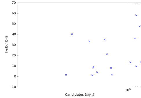
Fig. 3: The number of candidates per query subgraph compared with the ratio of Ti\&To / To-Ti .
