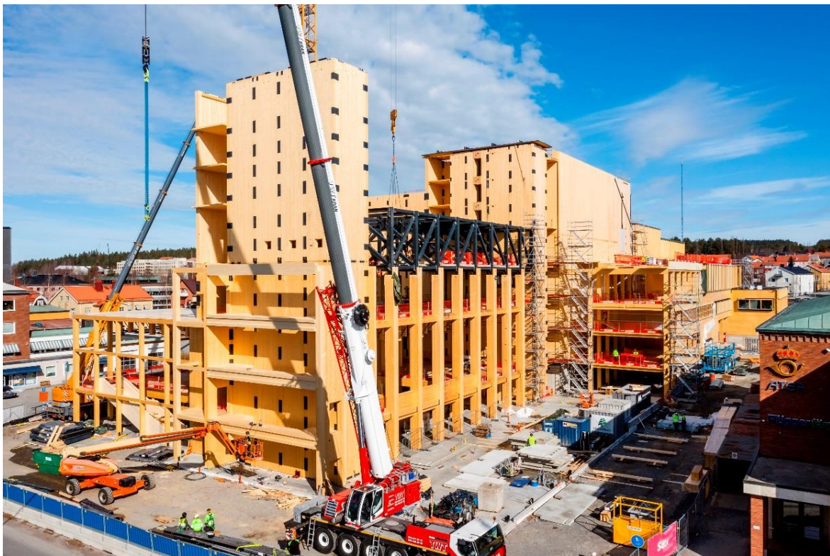
Figure 3.13 "Sara" Cultural Centre and Hotel in Skellefteå, Sweden will be 80 meters high and have 20 storeys. The total volume of the structure will be 10.000 m 3 CLT and 2200 m 3 glulam delivered by Martinsons. Photo: Jonas Westling (Sara, 2020)
