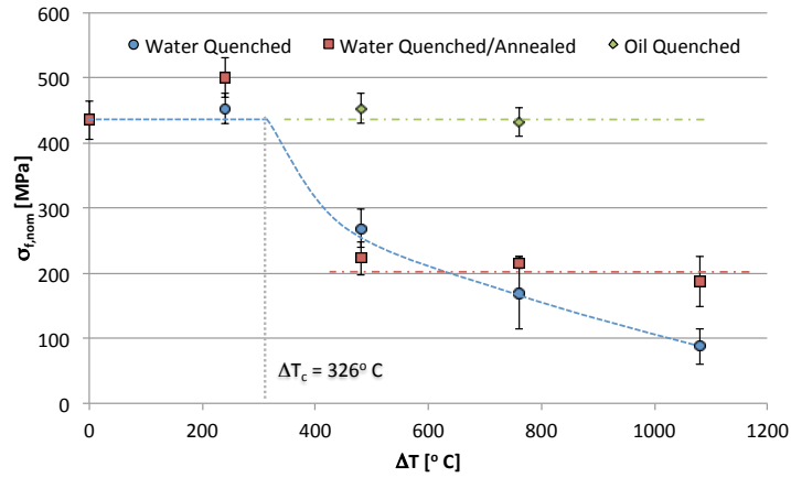
Figure 4: Flexural strength of PCBN A quenched in water and subsequent annealing from quench temperature as a function of quench temperature difference [\Delta T] .
