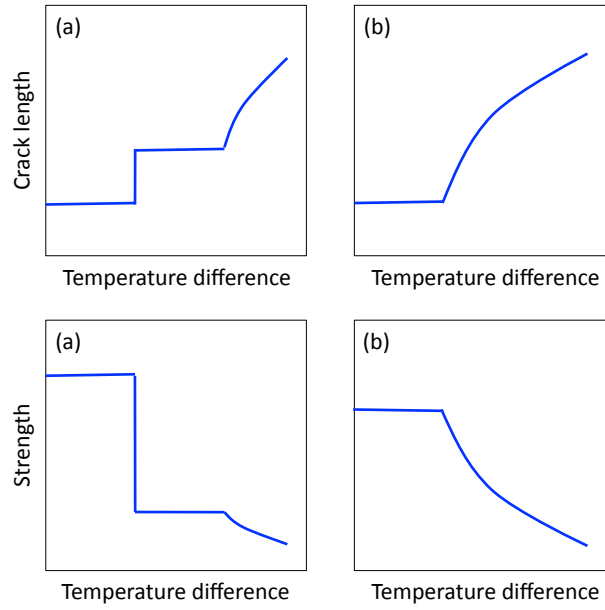
Figure 1: Crack propagation and strength for unstable (a) and stable (b) crack propagation conditions [5].
