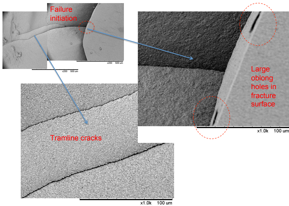
Figure 6: SEM Micrographs showing main features of quench failure of PCBN B.
