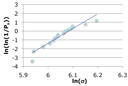
(a) PCBN A
