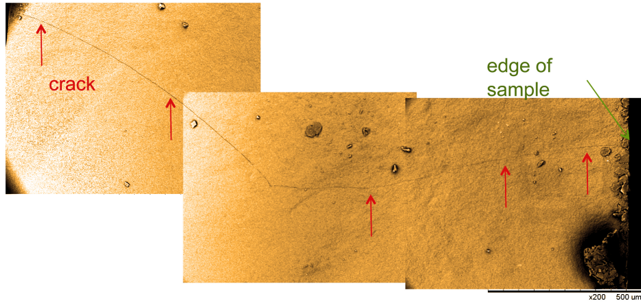
Figure 7: Knitted SEM micrograph of long unopened crack extending from failure initiation region to edge of sample.
