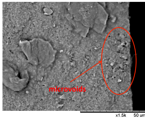
Figure 8: Fracture surface of PCBN B flexural strength sample, quenched from 1100° C. Microscopic voids are clearly evident close to the surface which are not present in the unquenched sample.
