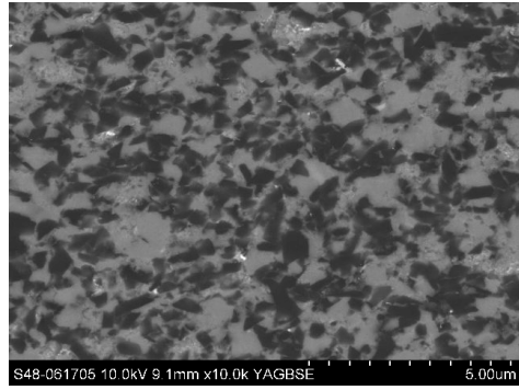
(b) PCBN B
