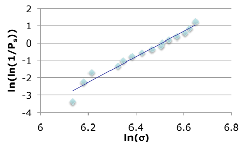
(b) PCBN B
