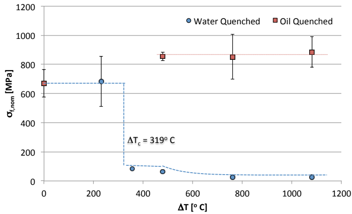
Figure 5: Flexural strength of PCBN B quenched in oil and water as a function of quench temperature difference [\Delta T] .
