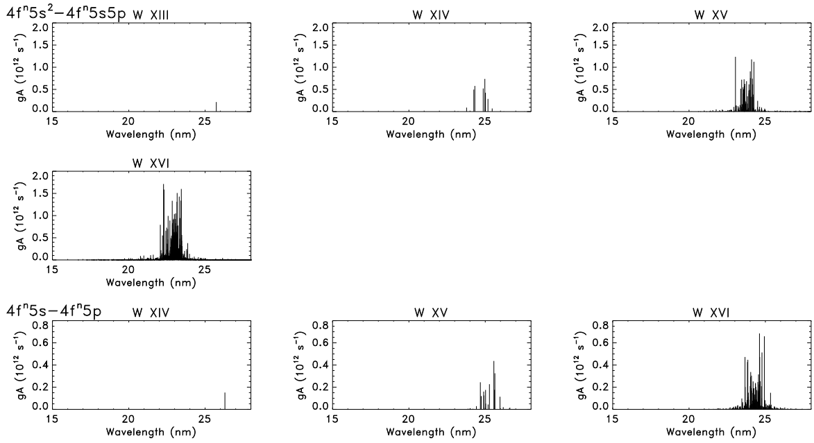
Figure 4. Calculated positions and gA values of 5s-5p_{1/2} transitions in W^{12+}-W^{15+} (W XIII–W XVI). The upper set correspond to 4f^n5s^2-4f^n5s5p ( n = 11-14 ), and the lower set to 4f^n5s-4f^n5p ( n = 12-14 ).
