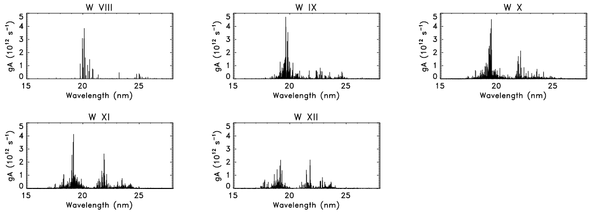
Figure 3. Calculated positions and gA values resulting from 5p-5d transitions in W^{7+}-W^{11+} (W VIII–W XII) corresponding to 4f^{14}5s^25p^n + 4f^{13}5s^25p^{n+1} - 4f^{14}5s^25p^{n-1}5d + 4f^{13}5s^25p^n5d ( n = 1-5 ).
