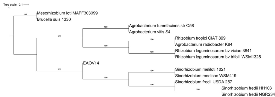
Figure 3 Phylogenetic reconstruction based on the concatenated 16S rRNA, 23S rRNA, atpD , chvA ( ndvA ), chvB , chvD , chvG ( exoS ), dnaK , exoC , gap , gyrB , infB , miaA , nusA pcs , pnp , recA , rpoB , and thrC gene sequences. Analyses were conducted using the consensus method (majority rule extended) with 100 bootstrap replicates. Bootstrap scores are represented numerically above branches. EAOV14 represents E. adhaerens .
