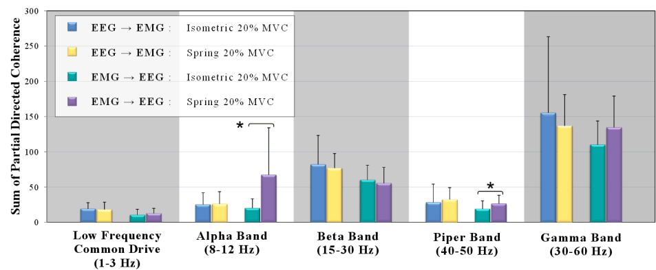
Figure 2. Bar plot comparing average PDC values and standard deviation for each subject in the low frequency, alpha, beta, piper and gamma frequency bands. A significant increase in alpha band coherence was observed in the EMG to EEG direction with the addition of the spring ( p = 0.0136 ). In the piper band, a significant increase in coherence is also detected for EMG to EEG ( p = 0.04695 ) direction.
