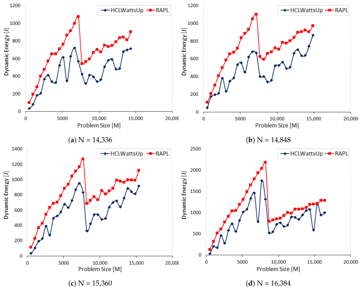
Figure 8. Dynamic energy consumption profiles of DGEMM on HCLServer01 and HCLServer02.
