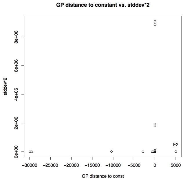
Fig. 4. GP performance difference to constant predictor versus double standard deviation of response variable in test set, for all 21 functions.
