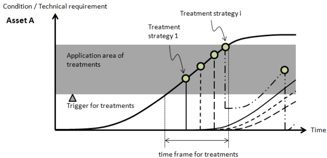
Figure 3 Deterioration and maintenance treatment strategy of asset A
