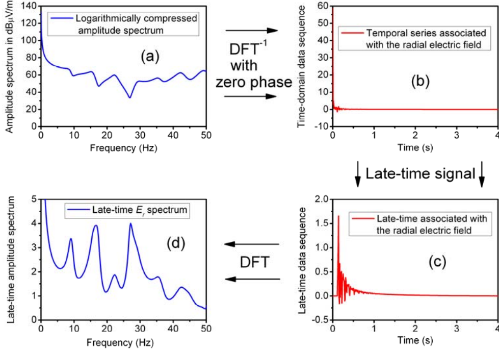
Figure 5. Analysis of the vertical component of electric field in the Earth's electromagnetic cavity.
