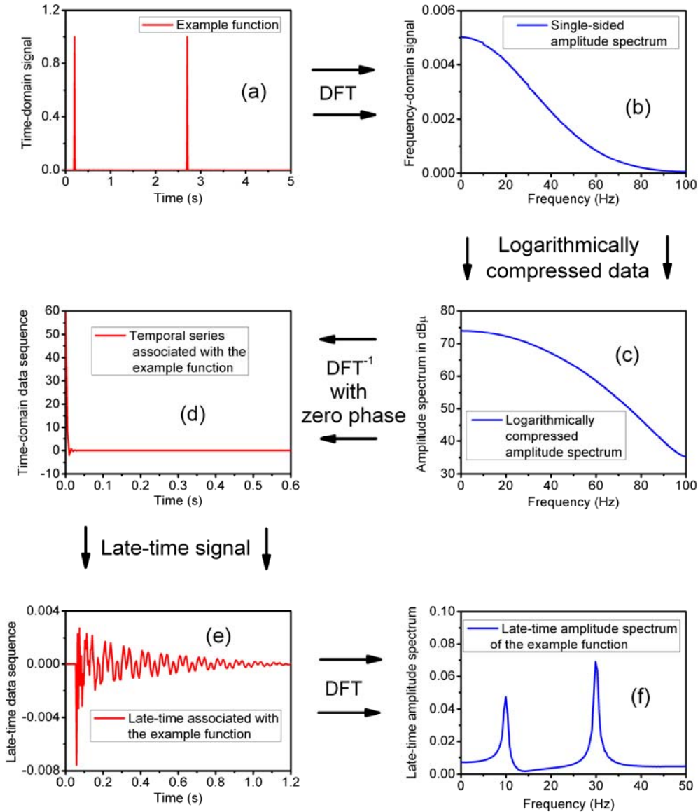
Figure 4. Different stages in the analysis procedure to extract weak resonances.
