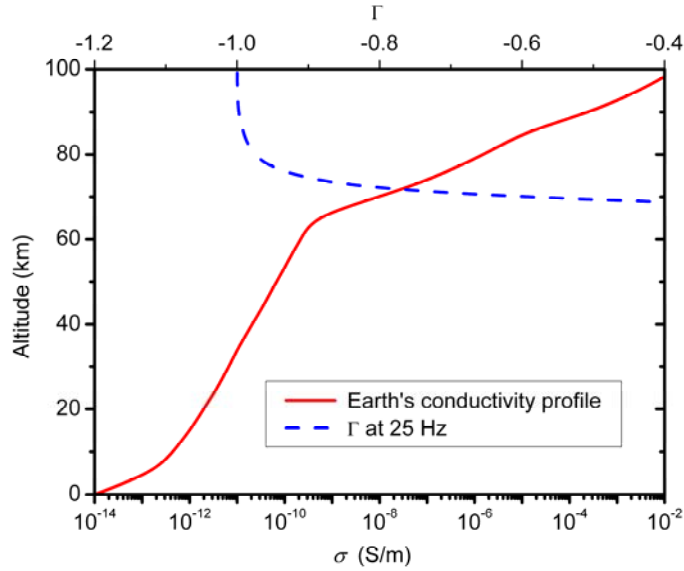
Figure 1. Conductivity and real part of the reflection coefficient profiles in the Earth's lower atmosphere.
