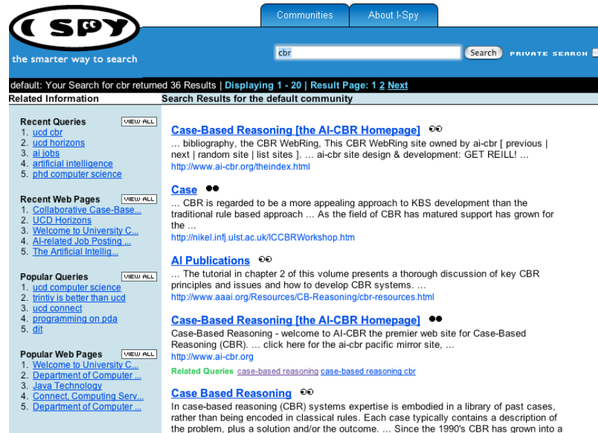
Fig. 6 An example I-Spy result-list showing a set of results retrieved for a given query. These results originate from underlying search engines such as Google and Bing but are re-ranked based on social search data, such as past selections for similar queries.
