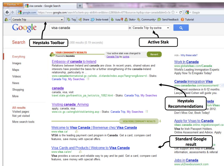
Fig. 8 An example of HeyStaks in action with Google. The HeyStaks toolbar is shown as a browser toolbar and provides the user with access to various features such as stak creation and sharing, and feedback options, such as voting and tagging. The screenshot shows a Google SERP that has been augmented with HeyStaks various augmentations, including a set of top-3 community promotions at the head of the Google result-list and annotations on regular Google results to indicate other community-relevant results.
