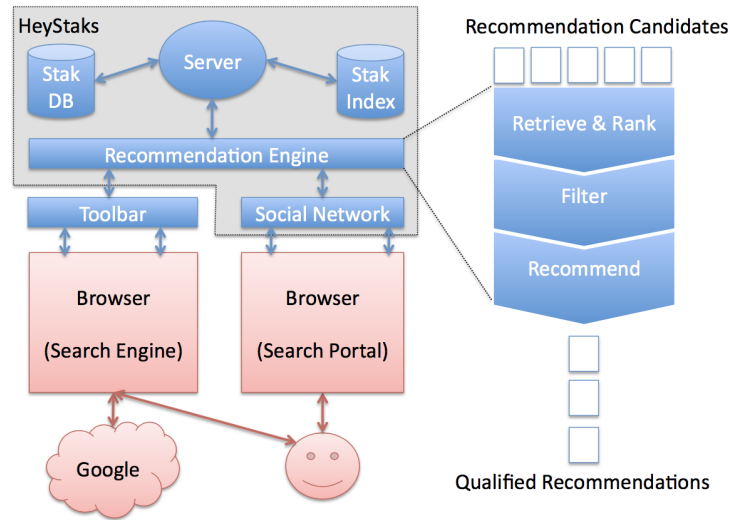
Fig. 7 HeyStaks is implemented as a back-end social search and recommendation system with a user-facing browser toolbar, thereby providing a seamless integration between HeyStaks and an existing search engine, such as Google.
