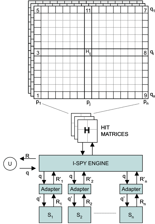
Fig. 5 The I-Spy system architecture showing the I-SPY collaborative search engine, search engine adaptors, and core hit-matrix as the basis for result relevance.
